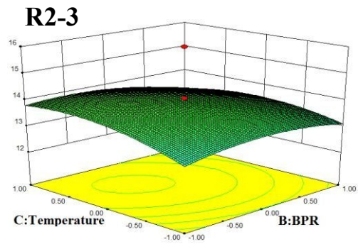
Figure 2S. Response surface for Flow rate, Column temperature and Back pressure.
