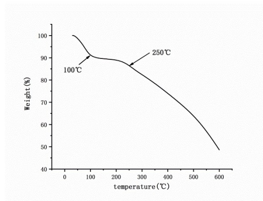
Fig. S2. TGA curves of PANI-HILs-Au coating.
