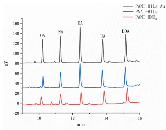
Fig. S3. Comparison of extraction effects of three coatings.
