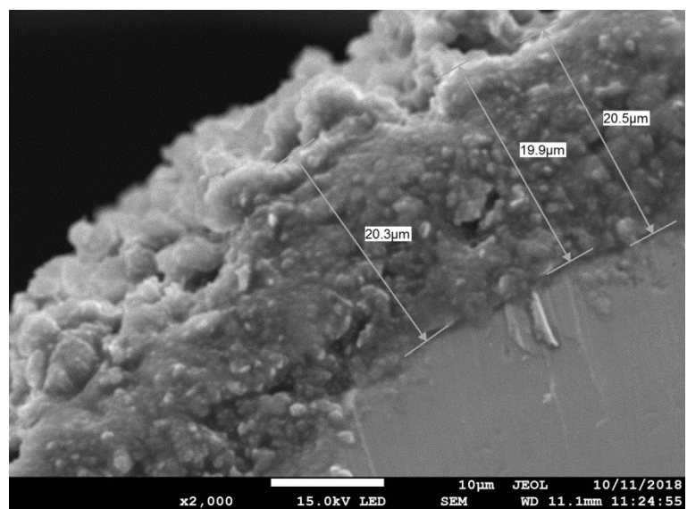
Fig. S1 The thickness of PANI-HILs-Au coating.
