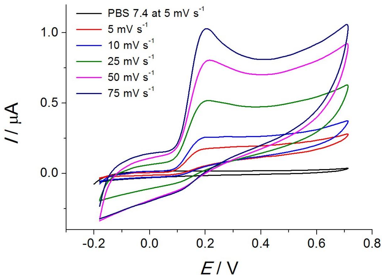
Fig. S1 Cyclic voltammograms of 25 µL Paeonia anomala L. on PGA/MWNT/GCE in phosphate buffer solution pH 7.4 at different potential scan rate.
