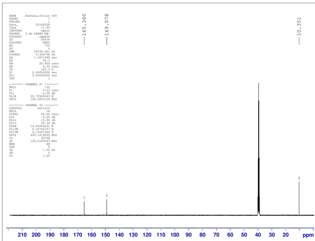
Fig. S2 13 C NMR spectrum of MMT.
