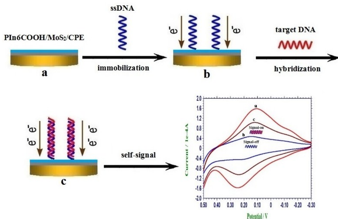
Scheme S1 The schematic illustration of the detection process and principle of the self-signal electrochemical sensing platform.
