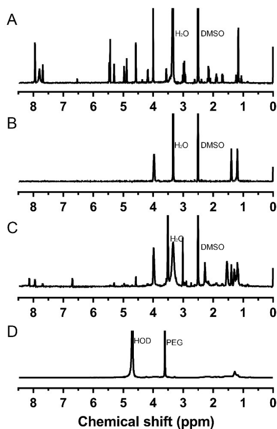
Fig.S1 1 H NMR spectra of DOX (A), DSF (B), DOX, DSF and PCL-PGlu-mPEG (C) in DMSO-d 6 , and Co-NPs-4 in D 2 O (D).
