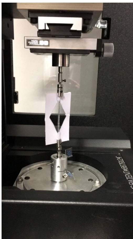
Figure S1. Picture of the apparatus and experimental set-up employed for the mechanical test.
