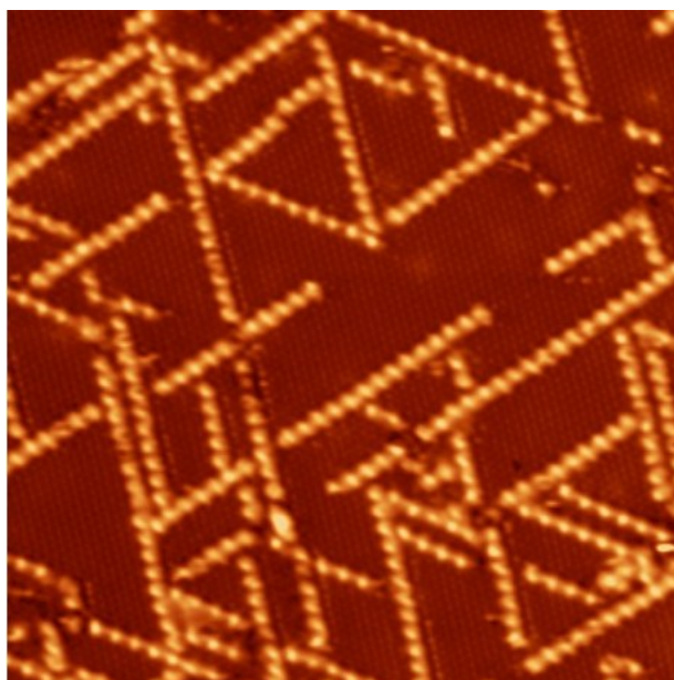
Fig. S1 STM image of NN lines on Si(111)-B ( 60 \times 60 \text{ nm}^2 , I_t = 10 \text{ pA} , V_s = -2.8 \text{ V} , T = 110 \text{ K} ).
