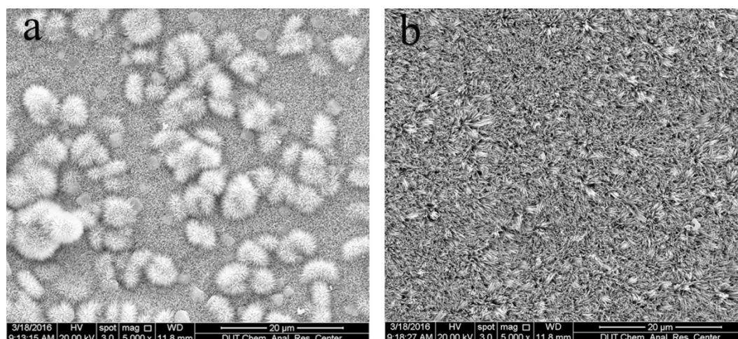
Fig. S2 SEM images of the Co-NWAs grown on the \alpha -Al 2 O 3 tubes treated (a) without or (b) with APTES treatment.
