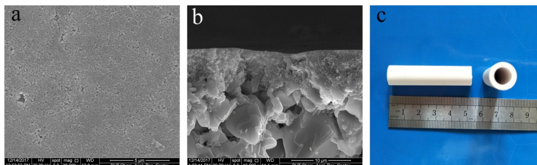
Fig. S1 SEM images of the surface of the \alpha -Al 2 O 3 tube. (a) Top view; (b) Cross-section view and (c) photograph of the \alpha -Al 2 O 3 tube.
