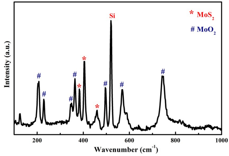
Fig. S1 Raman spectra of the microparticles in Figure 2(a) in the article.
