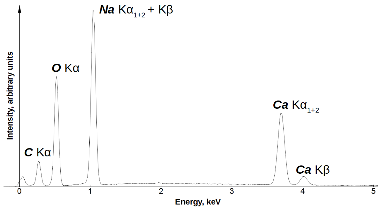
Figure S1. EDS spectrum of \text{Na}_4\text{Ca}(\text{CO}_3)_3
