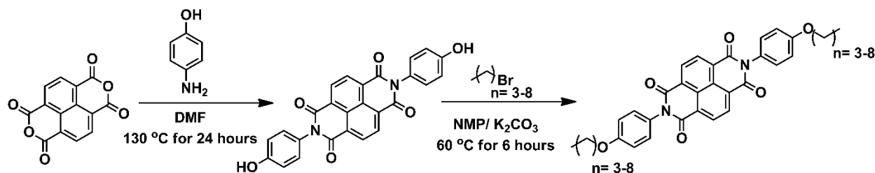
Scheme S1. Synthesis of alkoxyphenyl N-substituted naphthalene diimides discussed in this study.
