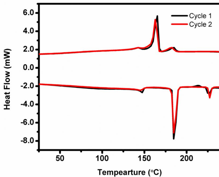
Figure S25. DSC curve for two consequent heating-cooling cycles of HxNDI
