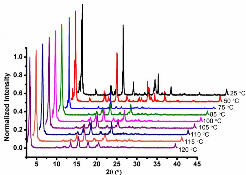
Figure S22. VTPXRD analysis of HNDI. Thermochromism occurs between 25 °C and 75 °C. At temperatures up to 75 °C, no significant changes were observed. Beyond 75 °C, changes to the 2\theta values occurred due to changes in the crystalline phase.
