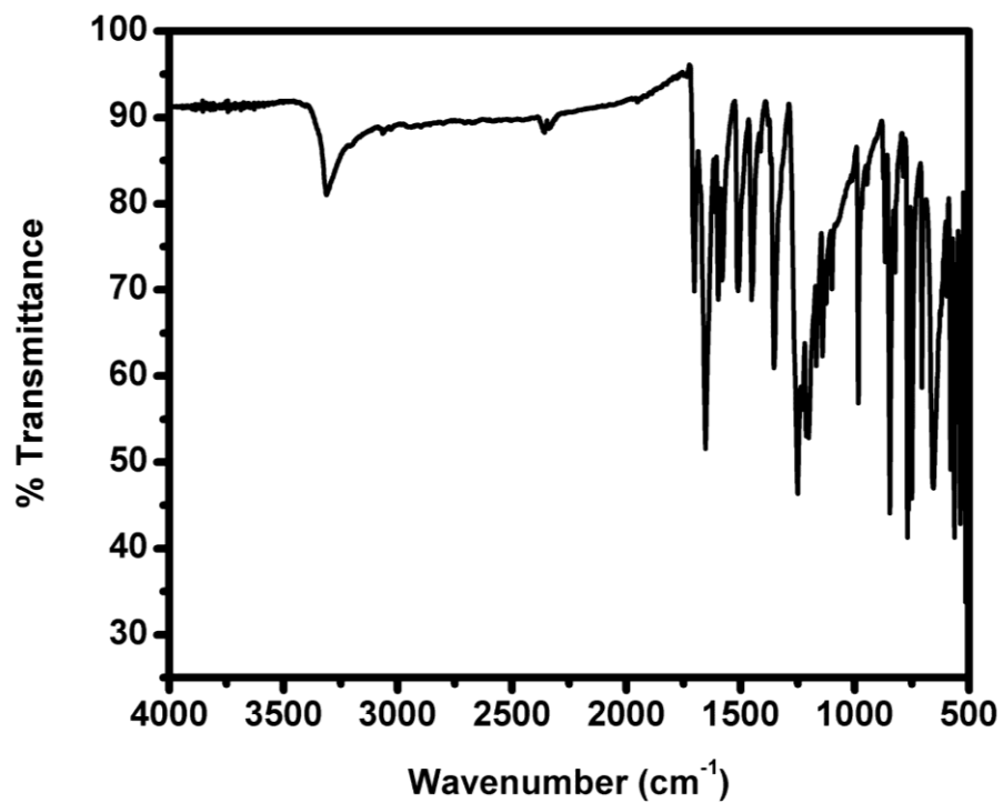
Figure S13. IR spectrum of NDI-Ph
