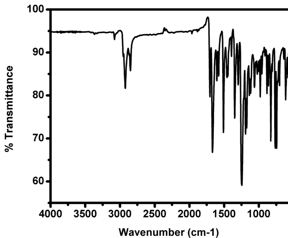
Figure S17. IR spectrum of ONDI
