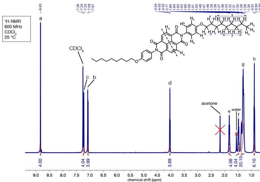
Figure S11: 1 H NMR spectrum of NNDI.
