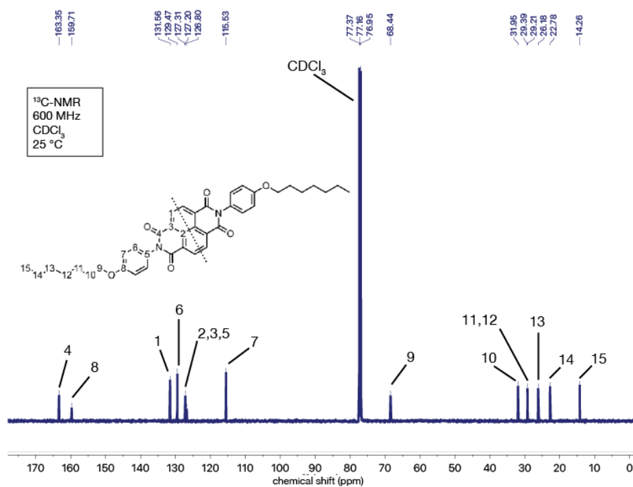
Figure S8: 13 C-NMR spectrum of HNDI.
