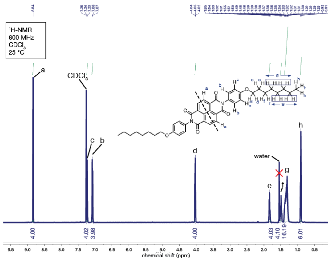
Figure S9: 1 H-NMR spectrum of ONDI.
