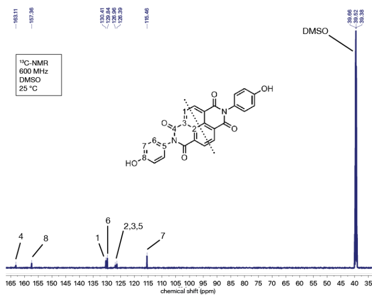
Figure S2: 13 C-NMR spectrum of NDI-Phenol.
