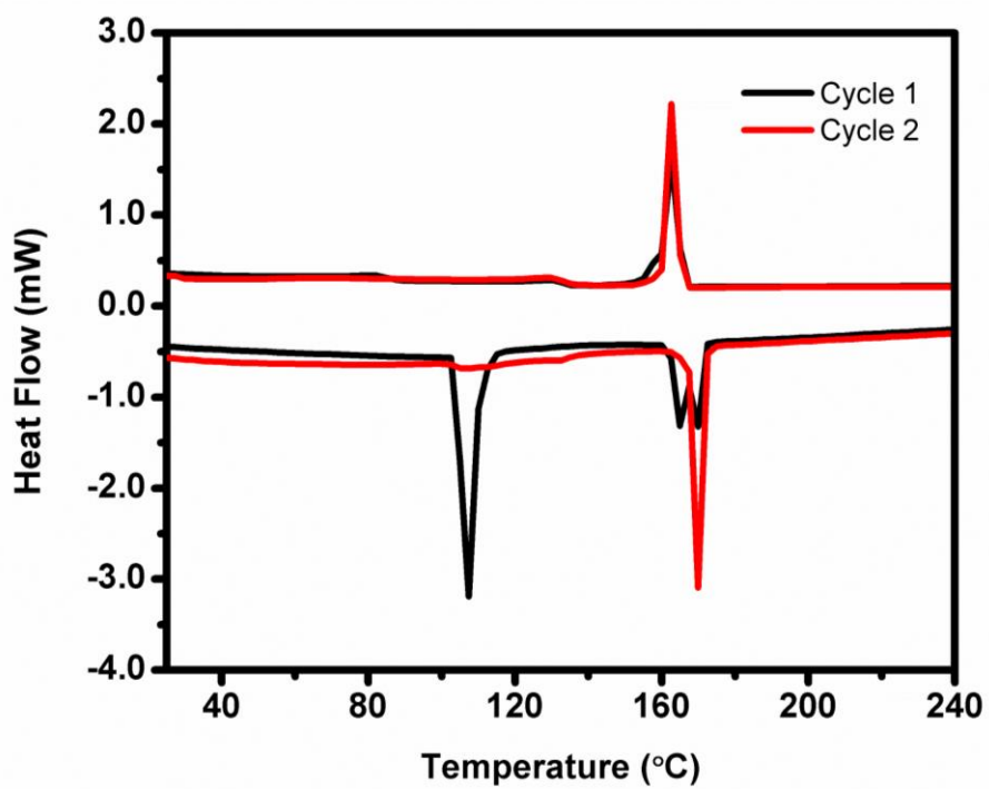
Figure S26. DSC curve for two consequent heating-cooling cycles of HxNDI
