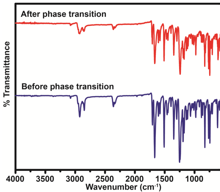
Figure S31. IR spectra of HNDI before and after irreversible phase transition
