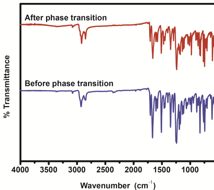
Figure S29. IR spectra of HNDI before and after irreversible phase transition
