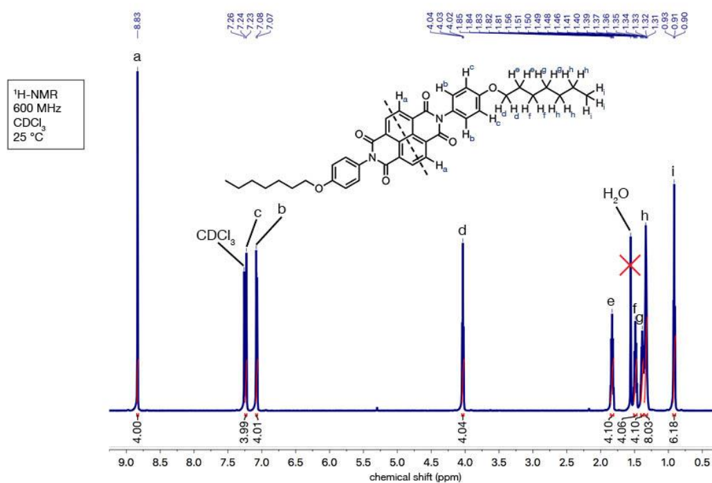
Figure S7: 1 H NMR spectrum of HNDI.
