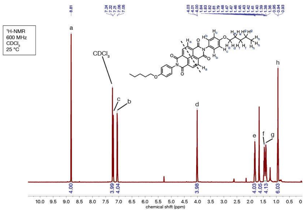
Figure S3: 1 H NMR spectrum of PNDI.
