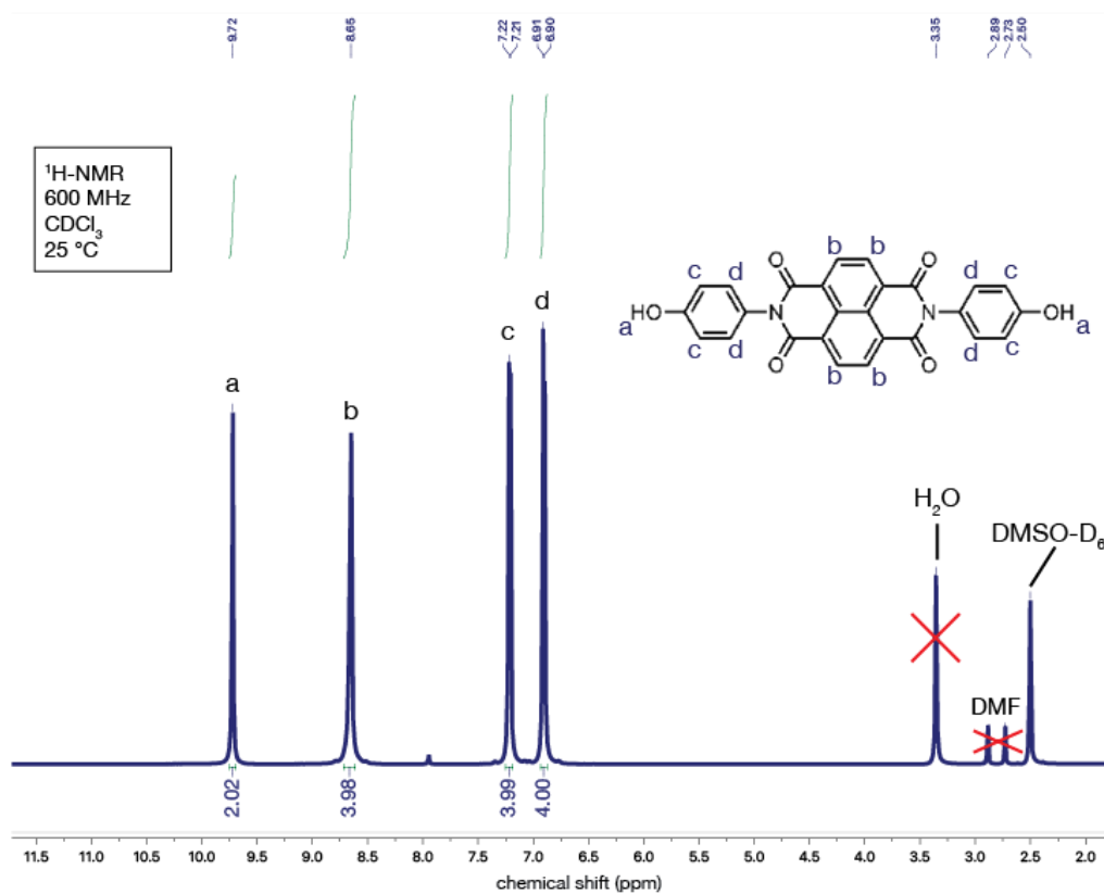
Figure S1: 1 H NMR spectrum of NDI-Ph.
