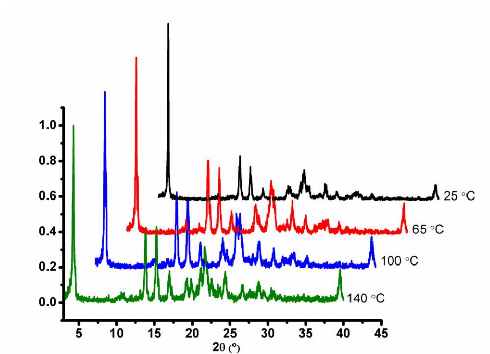
Figure S19. VTPXRD analysis of PNDI
