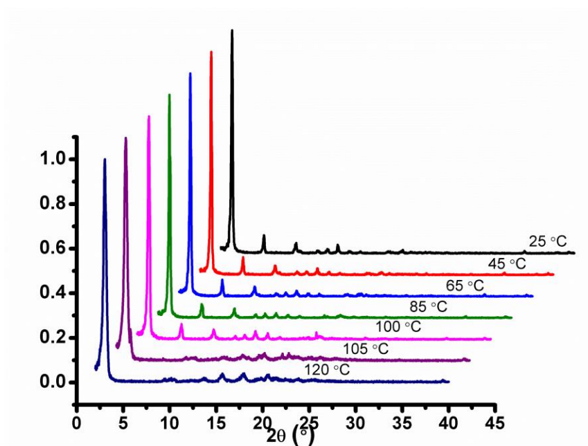
Figure S23. VTPXRD analysis of HNDI. Thermochromism occurs between 25 °C and 105 °C. At temperatures up to 105 °C, no significant changes were observed. Beyond 105 °C, changes to the 2\theta values occurred due to changes in the crystalline phase.
