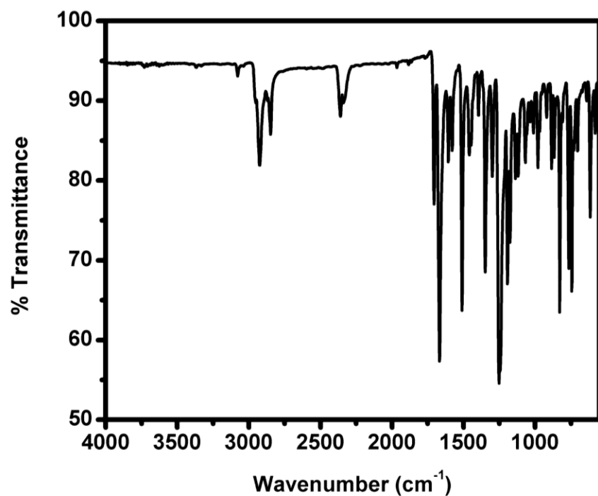
Figure S18. IR spectrum of NNDI. The signal observed near 2300 cm -1 is due to carbon dioxide in the atmosphere.
