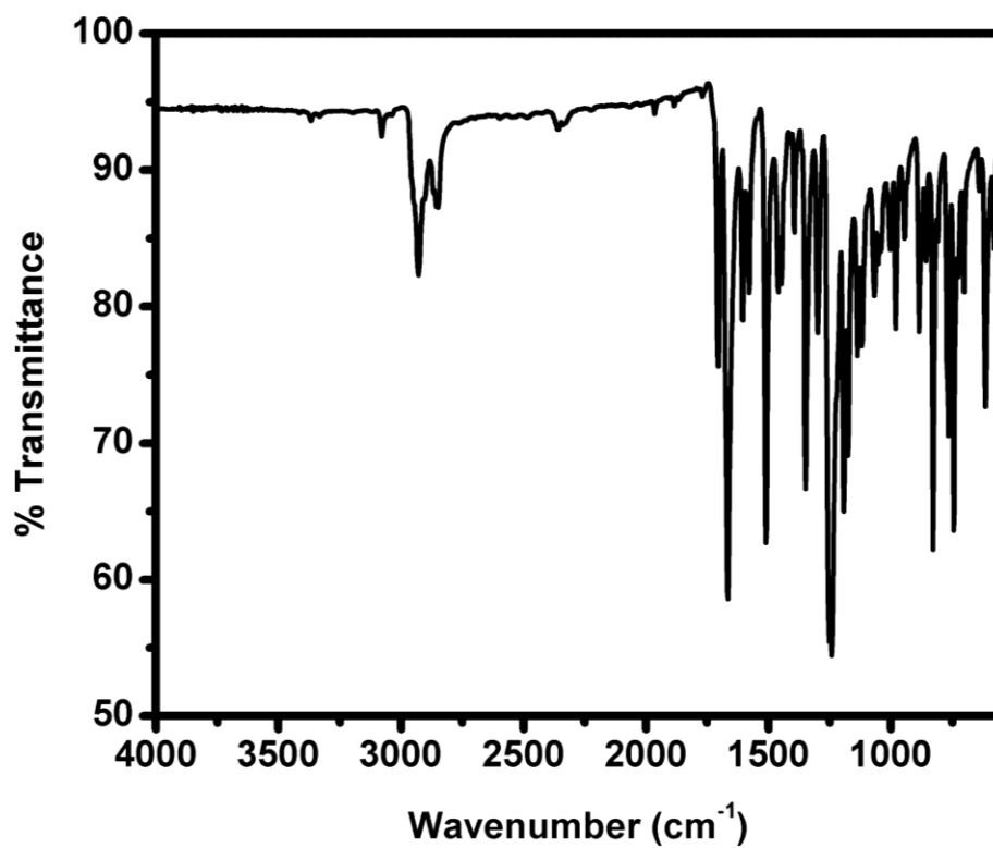
Figure S16. IR spectrum of HNDI
