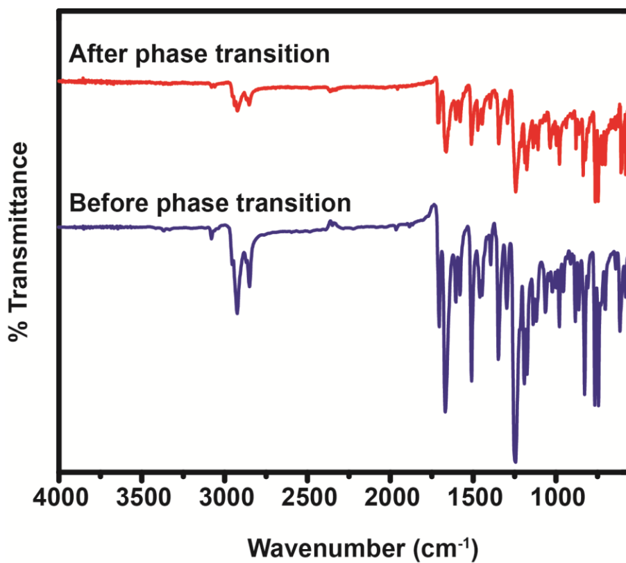
Figure S30. IR spectra of HNDI before and after irreversible phase transition
