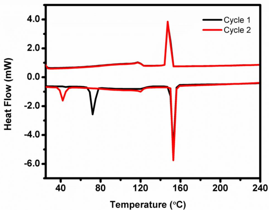
Figure S27. DSC curve for two consequent heating-cooling cycles of ONDI
