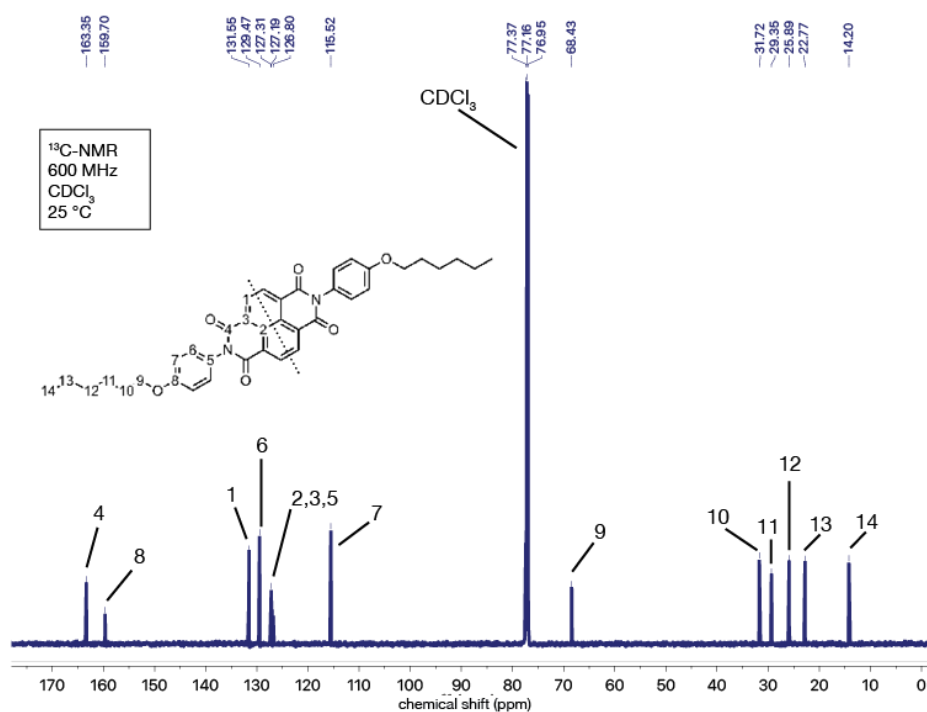
Figure S6: 13 C NMR spectrum of HxNDI.
