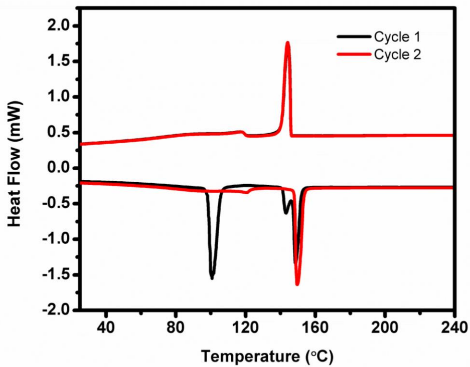
Figure S28. DSC curve for two consequent heating-cooling cycles of NNDI
