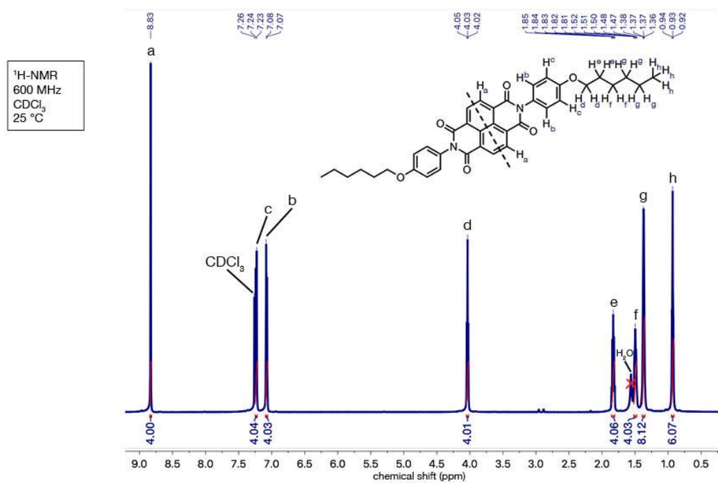
Figure S5: 1 H NMR spectrum of HxNDI.
