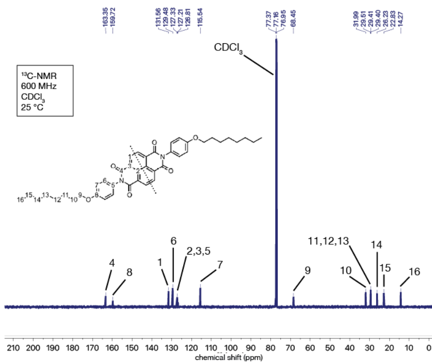
Figure S10: 13 C-NMR spectrum of ONDI.
