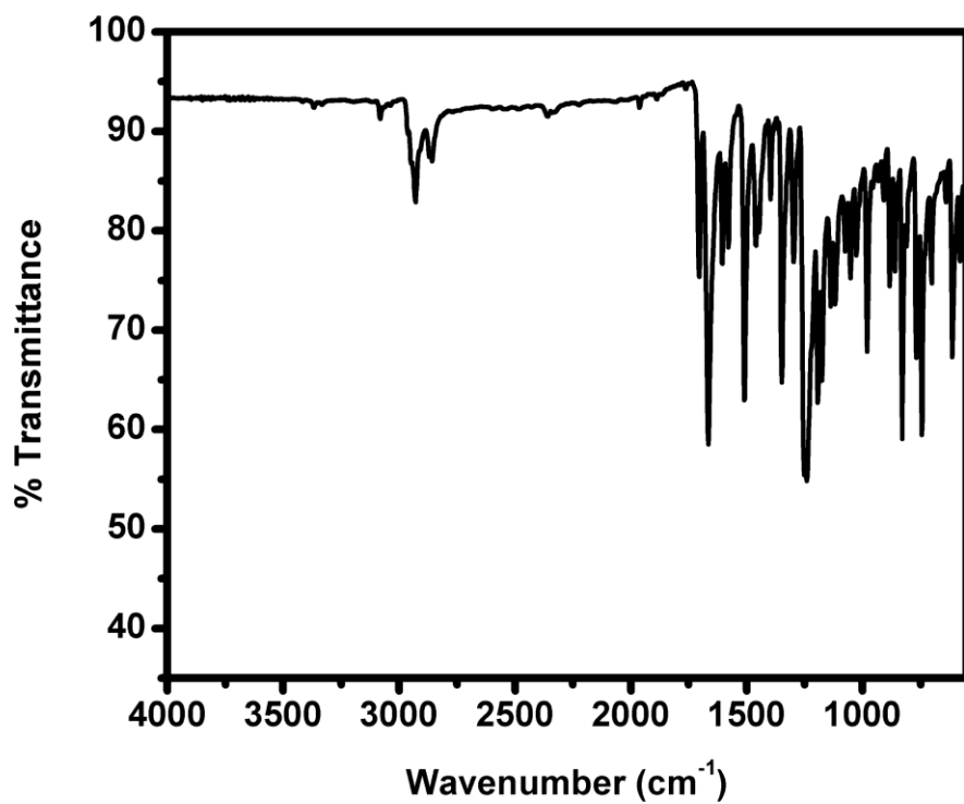
Figure S14. IR spectrum of PNDI
