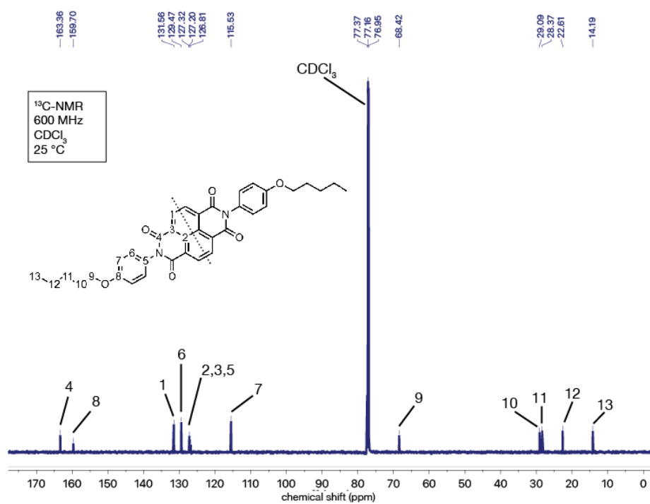
Figure S4: 13 C-NMR spectrum of PNDI.
