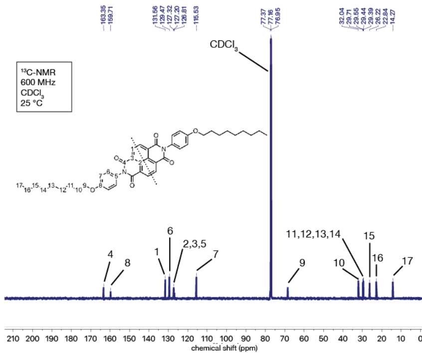
Figure S12: 13 C-NMR spectrum of NNDI.
