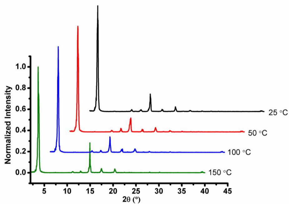
Figure S20. VTPXRD analysis of HxNDI
