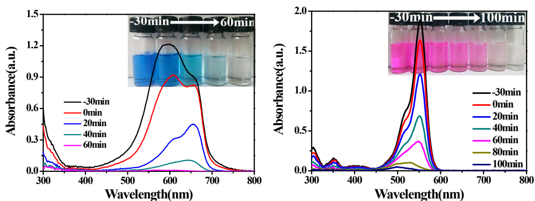
Figure S3 UV-vis absorption spectra of (a) MB (10 mg/L) and (b) RhB (10mg/L) using DS-2 as photocatalyst under visible light irradiation.
