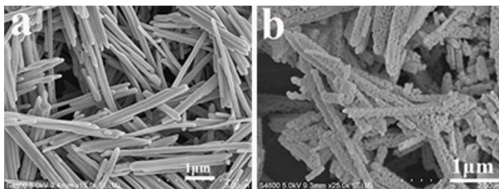
Figure S2 FE-SEM images of the \text{Bi}(\text{OHC}_2\text{O}_4)_2 \cdot 2\text{H}_2\text{O} (a), \text{Bi}_2\text{O}_3 (b).
