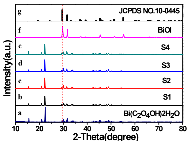
Figure S1. The XRD patterns of the precursors, (a) \text{Bi}(\text{OHC}_2\text{O}_4)_2 \cdot 2\text{H}_2\text{O} , (b) S-1, (c) S-2, (d) S-3 (e) S-4 (f) BiOI and (g) Standard Card of BiOI
