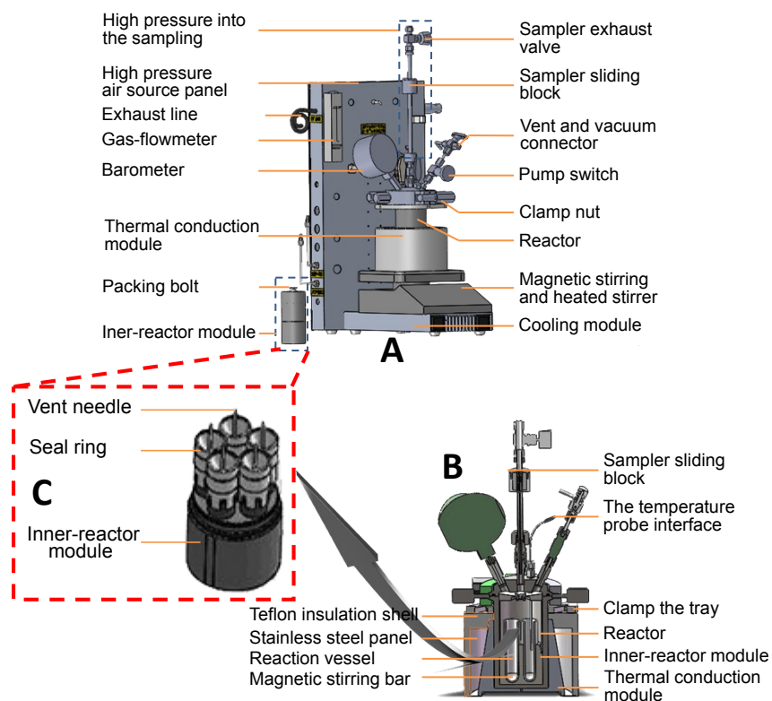
Scheme S1. (A) Over-view diagram, (B) section-view diagram, and (C) inner-reactor module diagram of the Wattecs Parallel Autoclave System (WPAS). 1
