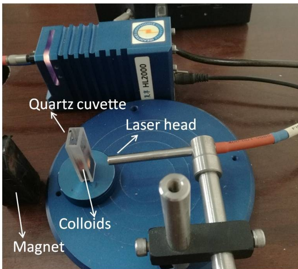
Fig. S3 Photo of reflection spectrum measurement of \text{Co}_x\text{Fe}_{3-x}\text{O}_4 suspension under magnetic field.
