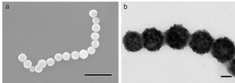
Fig. S2 Magnetic-field induced self-assembly of \text{Co}_{0.75}\text{Fe}_{2.25}\text{O}_4 . (a) SEM image. (b) TEM image. Scale bars, (a) 1\mu\text{m} , (b) 100\text{nm} .
