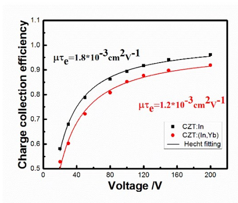
Figure S1 The hecht fitting results for CZT: In and CZT: (In, Yb)
