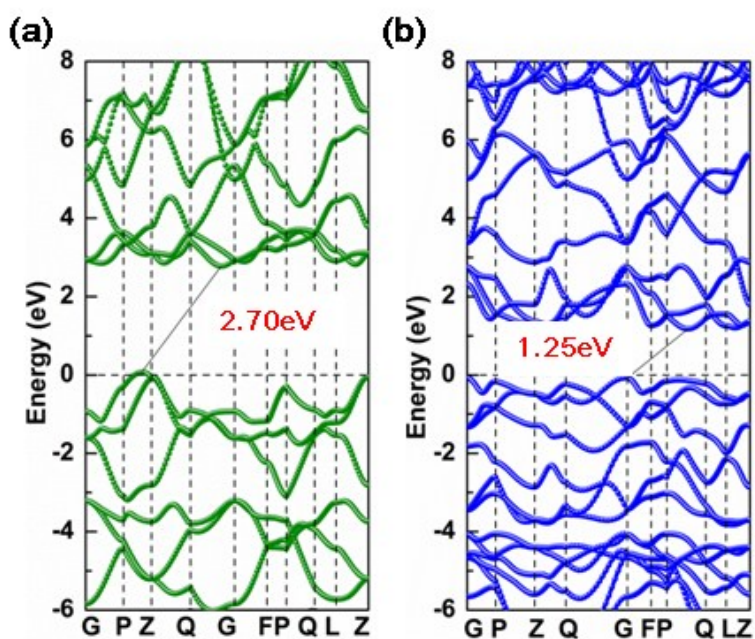
Figure S1 Electronic band structures along the high symmetry point in the Brillouin zone of Trig-C 9 (a) and Trig-C 15 (b) based on the HSE06 calculations
