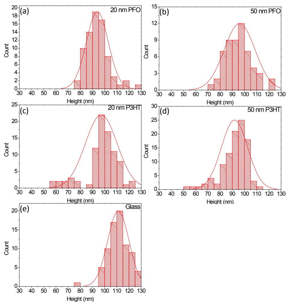
Figure S1. Histogram of the heights of AuNPs in the AuNP/polymer spacer/Au film system with various spacers: (a) 20 nm-thick PFO, (b) 50 nm-thick PFO, (c) 20 nm-thick P3HT, (d) 50 nm-thick P3HT, (e) AuNP directly on glass as a reference. Data were taken for at least 50 nm NPs in each case.
