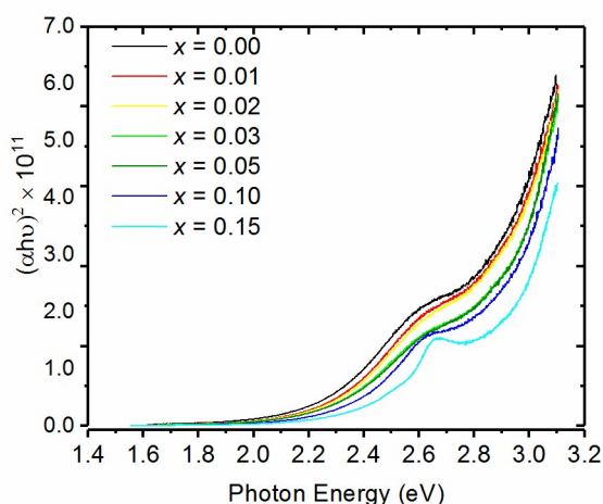
Figure S 1: Tauc plot obtained for the (\text{CH}_3\text{NH}_3)_{1-2x}(\text{H}_3\text{NC}_2\text{H}_4\text{NH}_3)_x\text{PbI}_3 system
