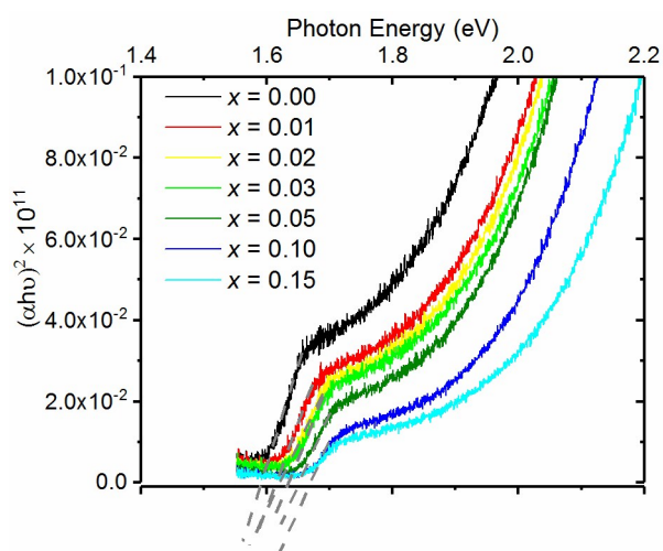
Figure S 2: Zoomed-in region of the Tauc Plot (shown in Figure S 1), showing regions fitted to obtain estimates of band gaps.
