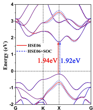
(a) a=3.118\text{\AA}
