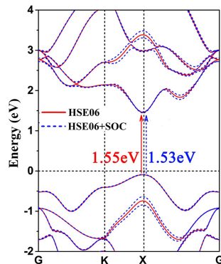
(f) a=3.168\text{\AA}
