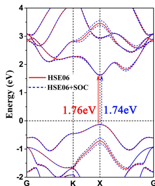
(c) a=3.138\text{\AA}
