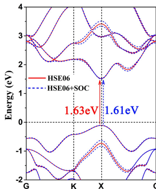
(e) a=3.158\text{\AA}
