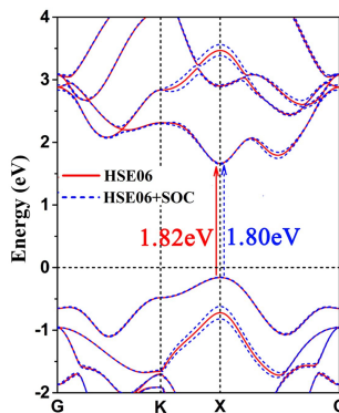
(b) a=3.128\text{\AA}
