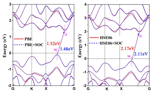
(a) a=3.118\text{Å}
