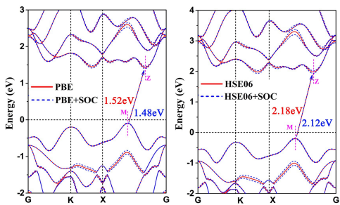
(b) a=3.128\text{Å}
