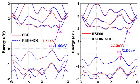
(e) a=3.158\text{Å}
