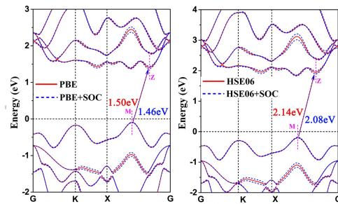
(f) a=3.168\text{Å}
