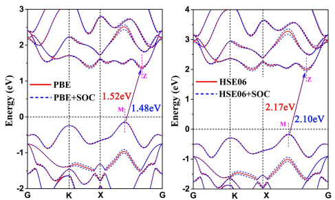
(c) a=3.138\text{Å}
