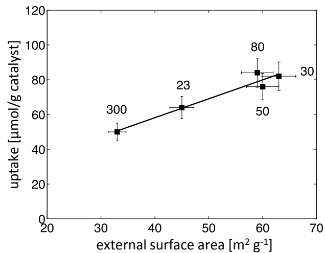
Figure S1. Correlation between collidine uptake and external surface area for HZSM5 samples with different SAR values.
