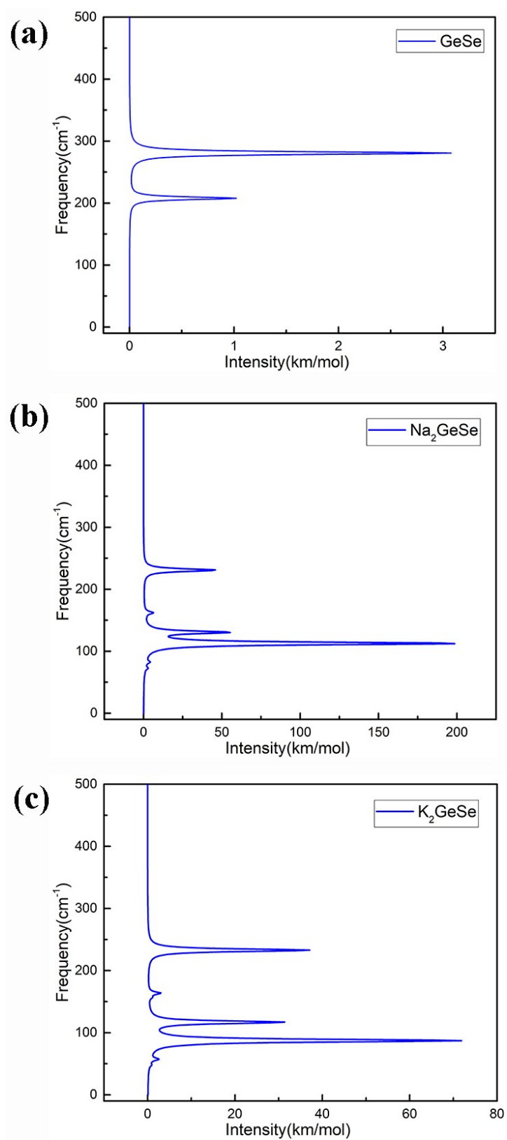
Figure S1. The frequency dispersion of the fully optimized (a) GeSe (b) Na 2 GeSe and (c) K 2 GeSe.
