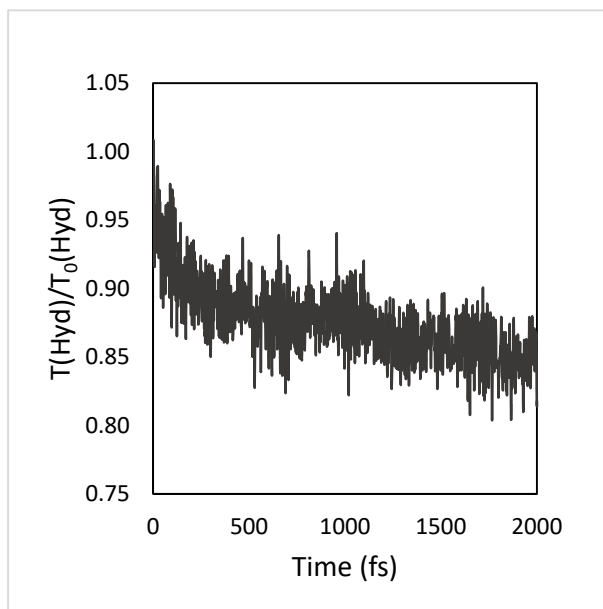
Figure S1. Average total kinetic energy of hydrogen atoms during the dynamics. The values are divided by the T(\text{Hyd}) at 0fs.
