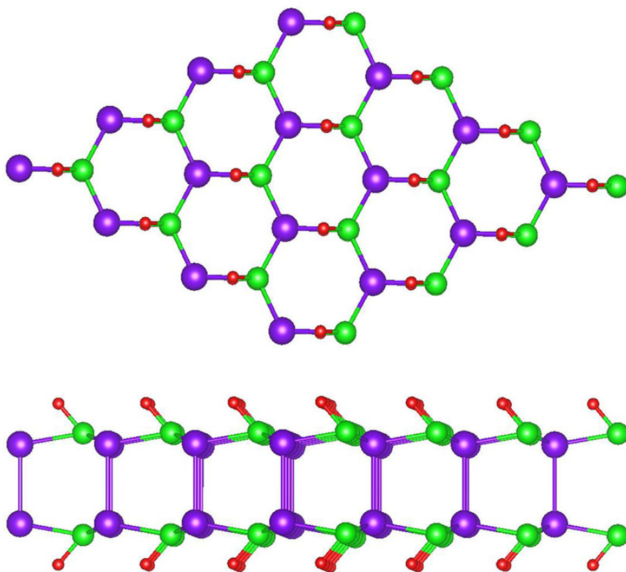
Fig. S1. Snapshots of atomic configuration at 2 ps for TlTeO at the end of MD simulation.
