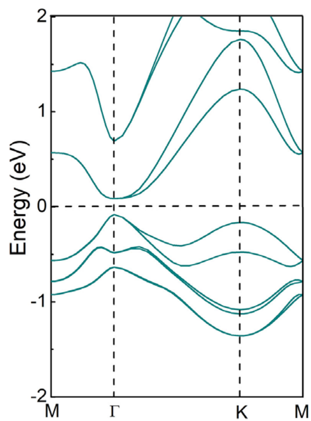
Fig. S2. The band structure of TlTeO by HSE06 with SOC.
