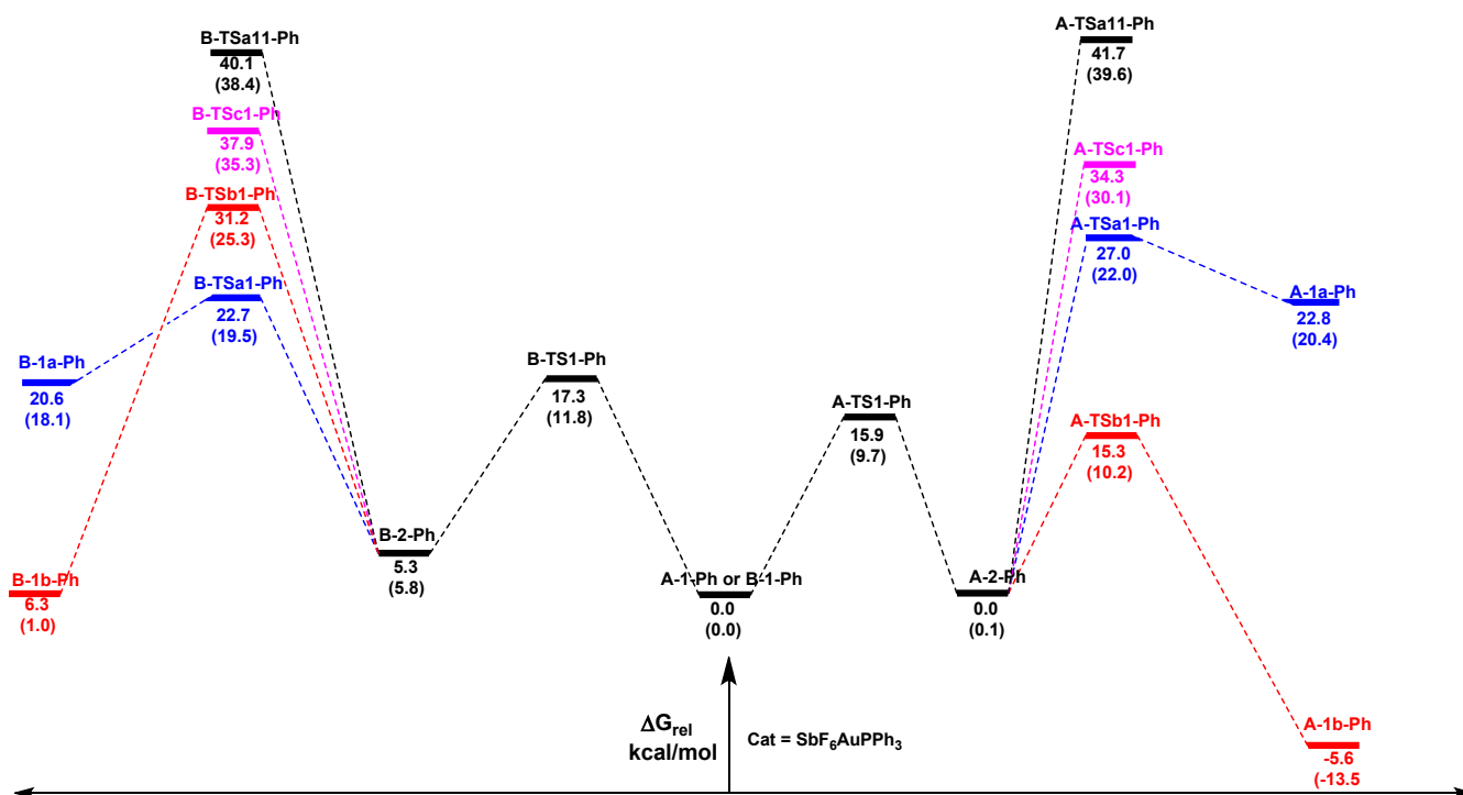
Figure S1. Energy profiles for the L=PPh_3 of path a , b and c , the relative energies are given in kcal/mol. These values were obtained at the M06-2X /SMD/6-311++G (d, p)//M06-2X /6-31G (d, p) level of theory. Values in brackets were obtained at the B3LYP-D3/SMD/6-311++G (d, p)//M06-2X /6-31G (d, p) level of theory.
