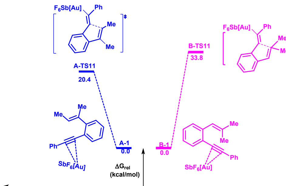
Figure S3. Energy profiles for 5- exo-dig for series A and B ; the relative energies are given in kcal/mol. These values were obtained at the M06-2X /SMD/6-311++G (d, p)/M06-2X /6-31G (d, p) level of theory.
