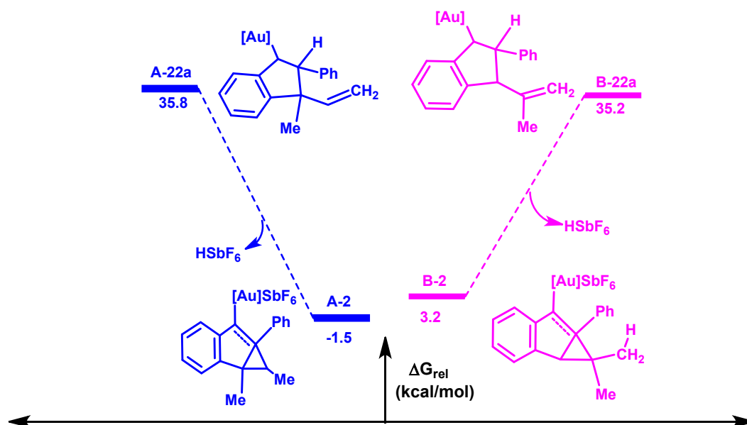
Figurer S2 Energy profiles for the formation of \text{HSbF}_6 ; the relative energies are given in kcal/mol. These values were obtained at the M06-2X /SMD/6-311++G (d, p)/M06-2X /6-31G (d, p) level of theory.
