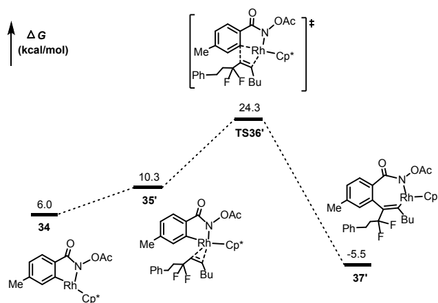
Fig. S8 Energy profiles for alkyne migratory insertion of 1a' and 2a.
