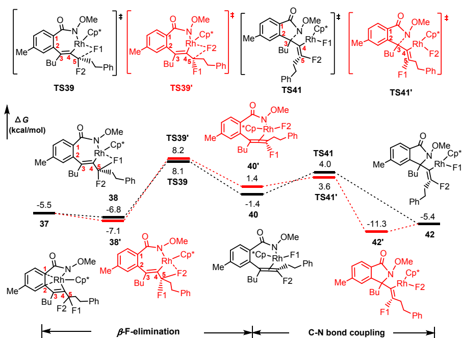
Fig. S9 The comparing pathway for β-F elimination at two different F (F1 or F2) sites.
