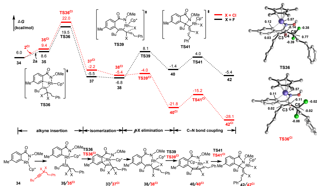
Fig. S10 Free energy profiles for the comparisons between different alkyne substrates ( 2a or 2Cl ) and N -methoxyl benzamide 1a' .
