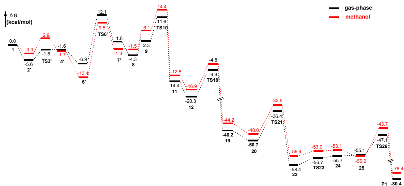
Fig. S1 Free energy profiles for the optimal path for hydroarylation products P1.
