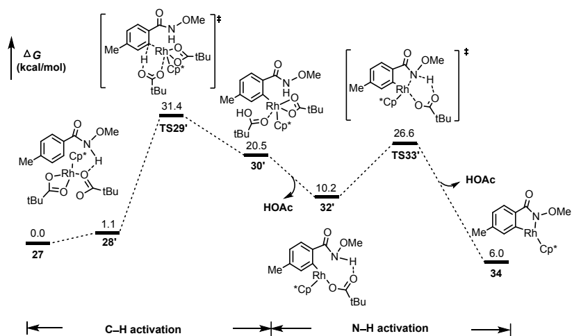
Fig. S7 Energy profiles for C–H activation, N–H deprotonation sequences of 1a'.
