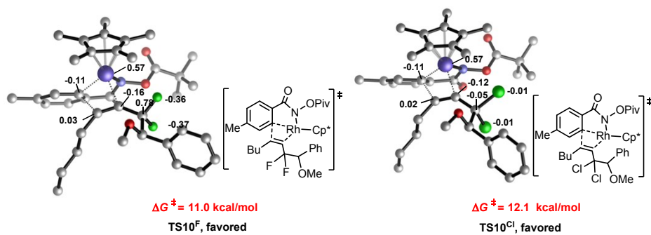
Fig. S11 Free energy profiles for alkyne insertion with different different alkyne substrates ( 2'a or 2'Cl ) in hydroarylation process.
