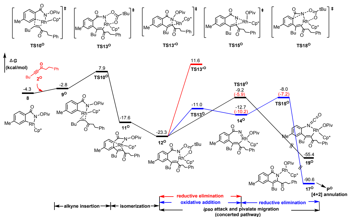
Fig. S5 Free energy profiles for the alkyne insertion and the competing pathways for the formation of 17^\circ or 19^\circ . Numbers in parentheses are relative free energies by optimization in MeOH (To get more accurate energies, some key structures were optimized in solvent).
