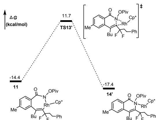
Fig. S2 Free energy profiles for direct C—N reductive elimination of 1a and 2a.
