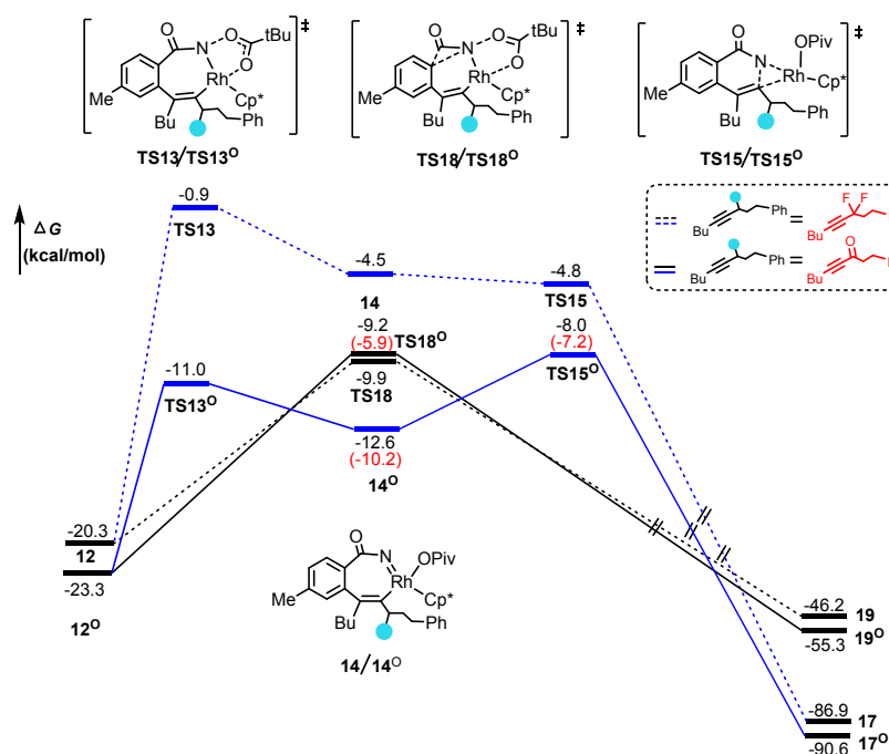
Fig. S6 Free energy profiles for the comparisons between different alkyne substrates ( 2a or 2° ) and N -pivaloyloxy benzamide 1a . Numbers in parentheses are relative free energies by optimization in MeOH solution.
