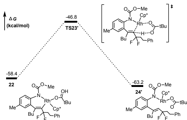
Fig. S4 Free-energy profiles for C—H protonated from 22.
