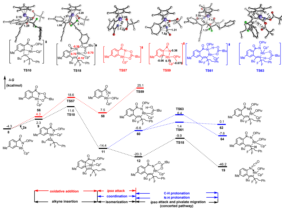
Fig. S3 Free energy profiles for Lossen rearrangement before the alkyne insertion or protonation of 11.
