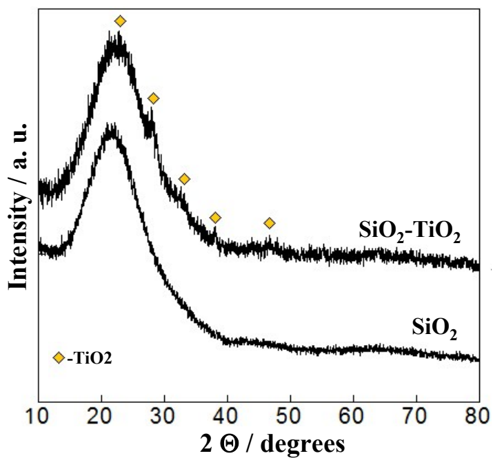
S1 Comparative XRD pattern of tubular \text{SiO}_2 and of \text{SiO}_2\text{-TiO}_2 composite.
