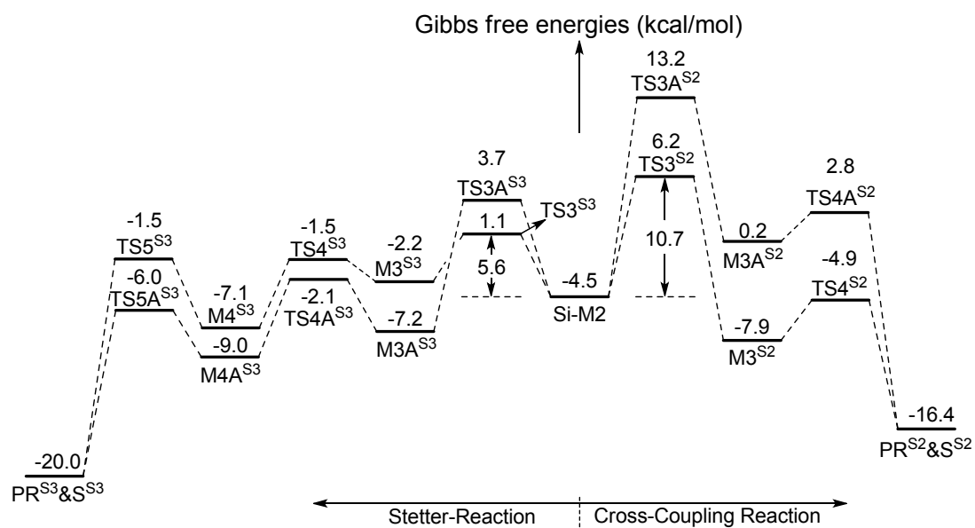
Fig. S6 The entire energy profiles of Cross-Coupling and Stetter reactions (Energy in kcal/mol)
