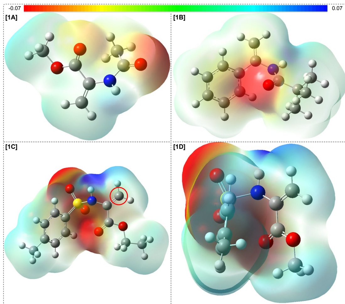
Fig. S1 Electron cloud distribution of the four representative 2-aminoacrylates
