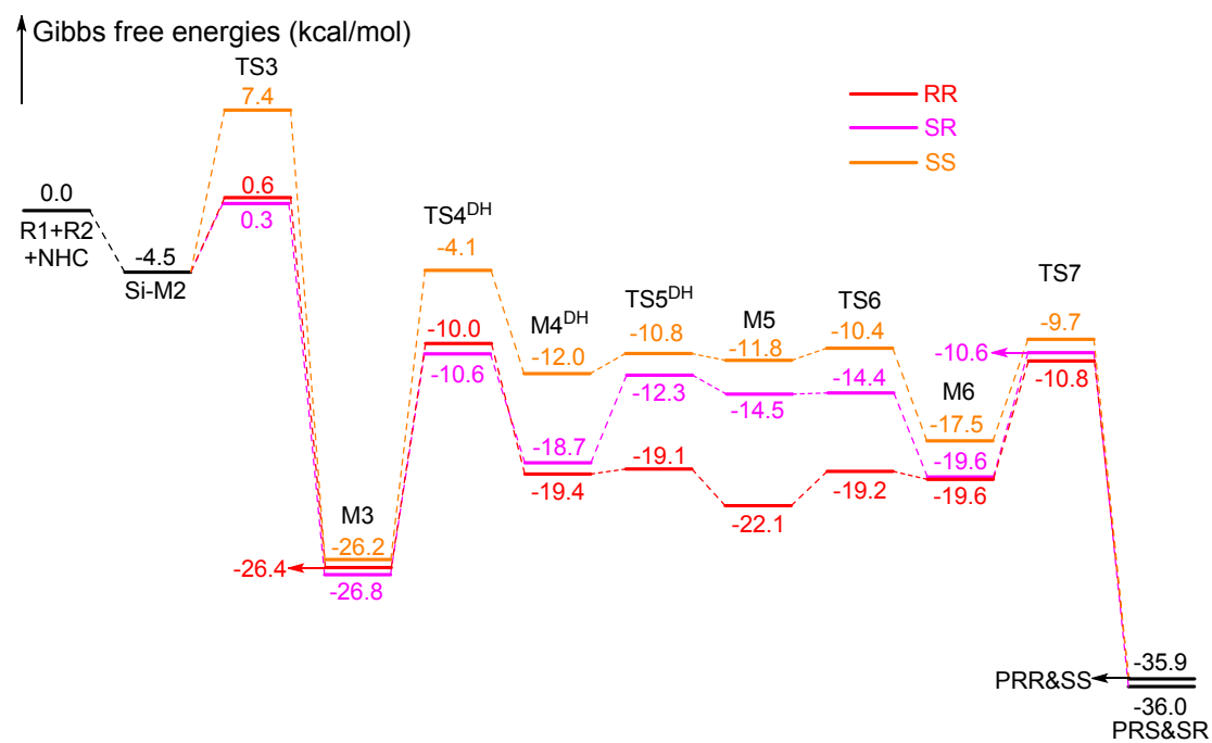
Fig. S3 The energy profile of [3 + 2] annulation reaction involved in another three pathways
