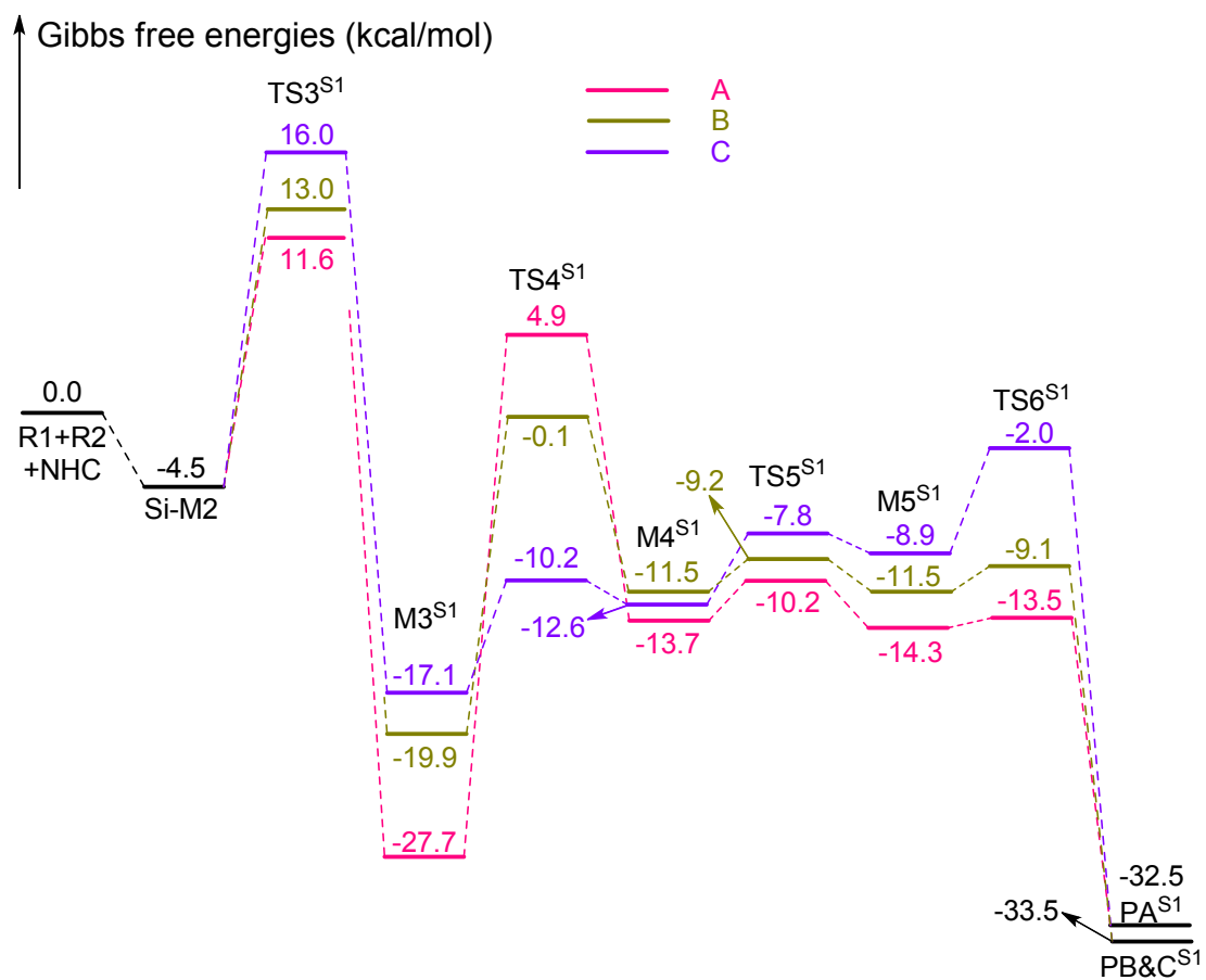
Fig. S5 The energy profile of [3 + 3] annulation reaction involved in another three pathways
