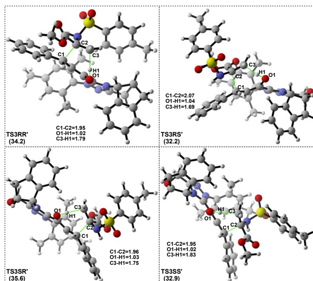
Fig. S2 3D-structures and energy barriers of transition states involved in the reaction pathway between 2-aminoacrylate R2 and Breslow intermediate Si-M2 (Distance in Å and energy in kcal/mol)
