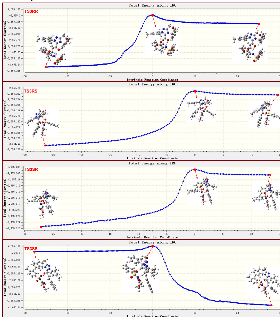
Fig. S4 IRC plots of stereochemical transition states
