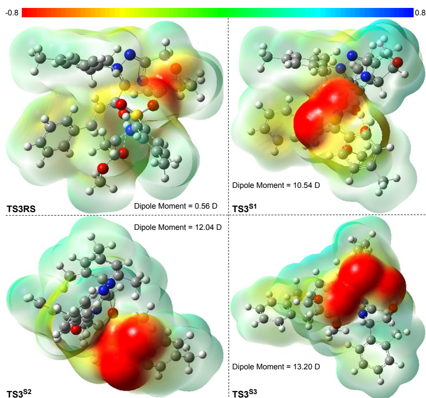
Fig. S7 The electrostatic potential surface of the chemoselective transition states TS3 , TS3 S1 , TS3 S2 , and TS3 S3
