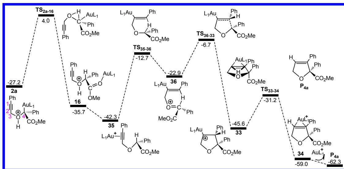
Fig. S4 Calculated free energy profile in DCE solvent along the possible pathway for forming product P 4a starting from 2a . The relative free energies are given in kcal mol -1 .
