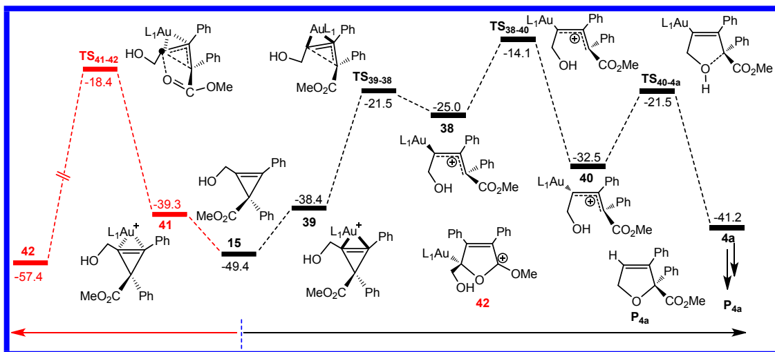
Fig. S6 Calculated free energy profiles in DCE along two possible pathways bifurcated from 15 . The relative free energies are given in kcal mol -1 .
