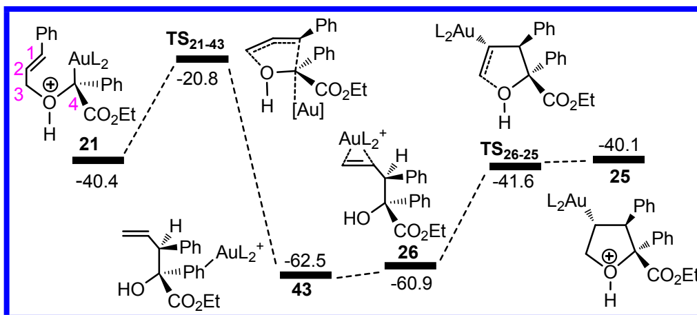
Fig. S7 Calculated free energy profile in Et 2 O solvent along the possible pathway via [2,3]-σ rearrangement for step 21 → 25 . The relative free energies are given in kcal mol -1 .
