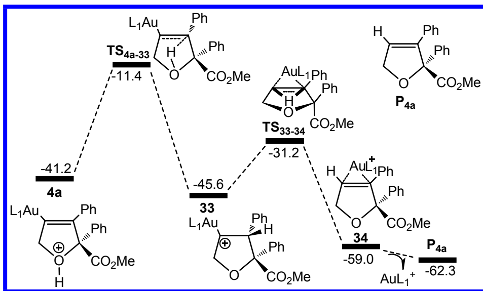
Fig. S1 Calculated free energy profile in DCE solvent for the 4a → P 4a transformation via the direct [1,3]-H shift. The relative free energies are given in kcal mol -1 . L 1 = JohnPhos
