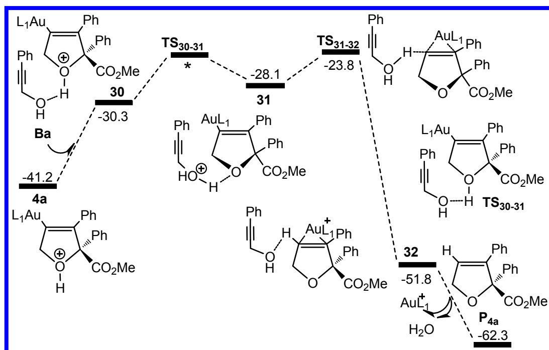
Fig. S2 Calculated free energy profile in DCE solvent for the 4a → P 4a transformation via the Ba -assisted [1,3]-H shift. The relative free energies are given in kcal mol -1 . L 1 = JohnPhos
