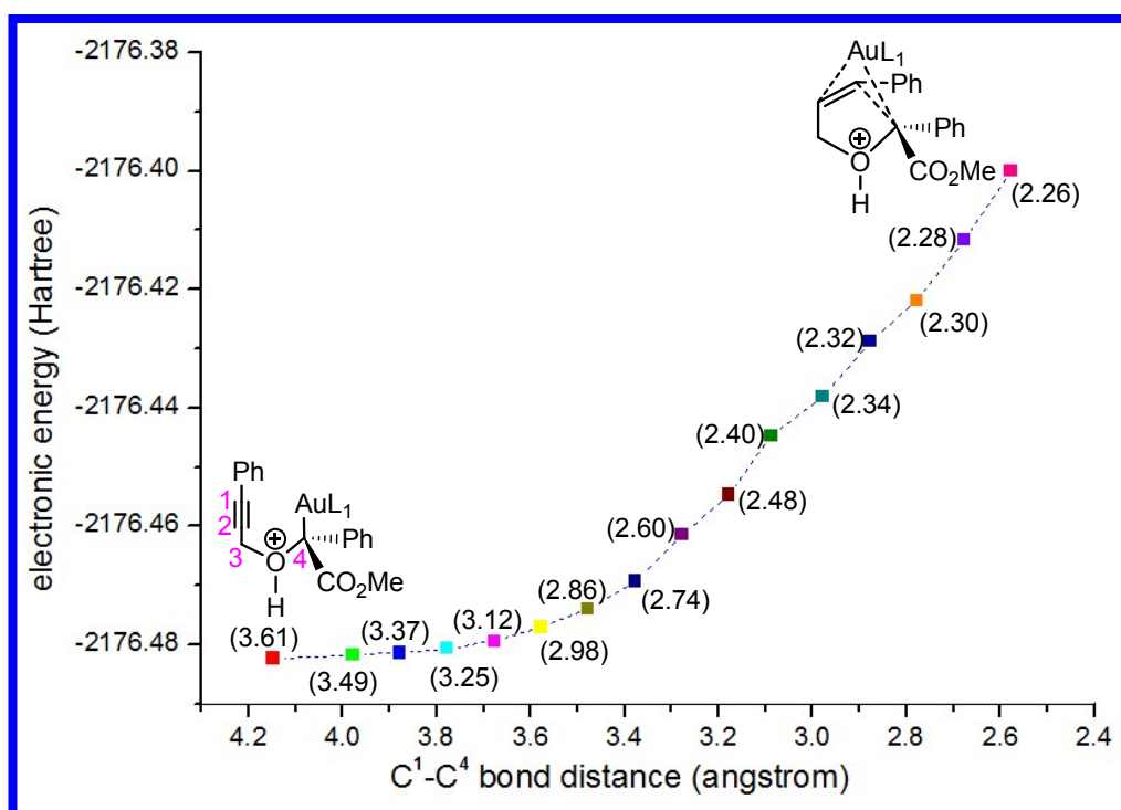
Fig. S3 Relax energy surface scan of the C 1 -C 4 bond distances for the transition state TS 2a-4a along the IRC curve. The values in parentheses are the Au-C 2 bond distances.
