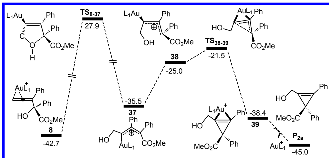
Fig. S5 Calculated free energy profile in DCE solvent along the possible pathway for forming product P 2a starting from 8 . The relative free energies are given in kcal mol -1 .
