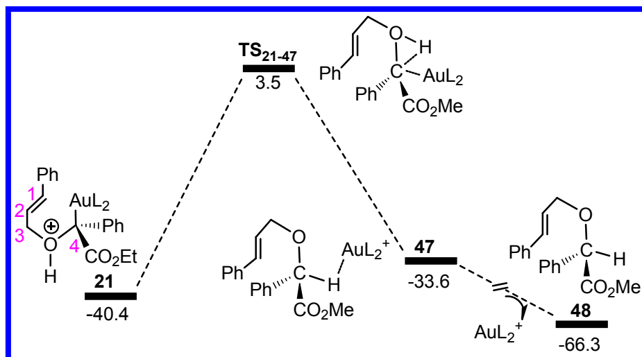
Fig. S9 Calculated free energy profile in Et 2 O solvent along the possible pathway for [1,2]-H shift of intermediate 21 . The relative free energies are given in kcal mol -1 .
