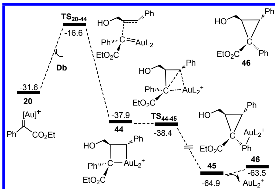
Fig. S8 Calculated free energy profile in Et 2 O solvent along the possible pathway starting from 20 . The relative free energies are given in kcal mol -1 .
