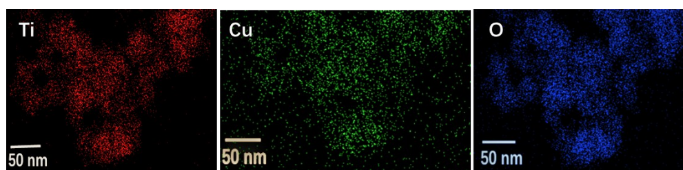
Fig. S2 EDX mapping images of 20wt% CuO/TiO 2 .
