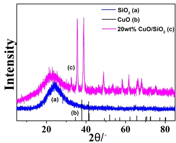
Fig. S1 XRD diffraction patterns of (a) \text{SiO}_2 ; (b) \text{CuO} ; (c) 20wt% \text{CuO}/\text{SiO}_2 nanocomposite.
