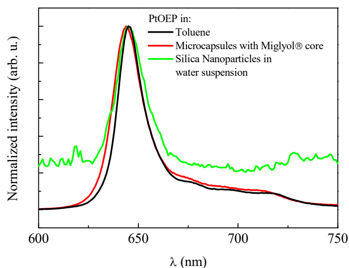
Figure S1. Normalized emission spectra of PtOEP in different environment. Spectra recorded in nitrogen atmosphere. \lambda_{\text{exc}} = 535 nm.
