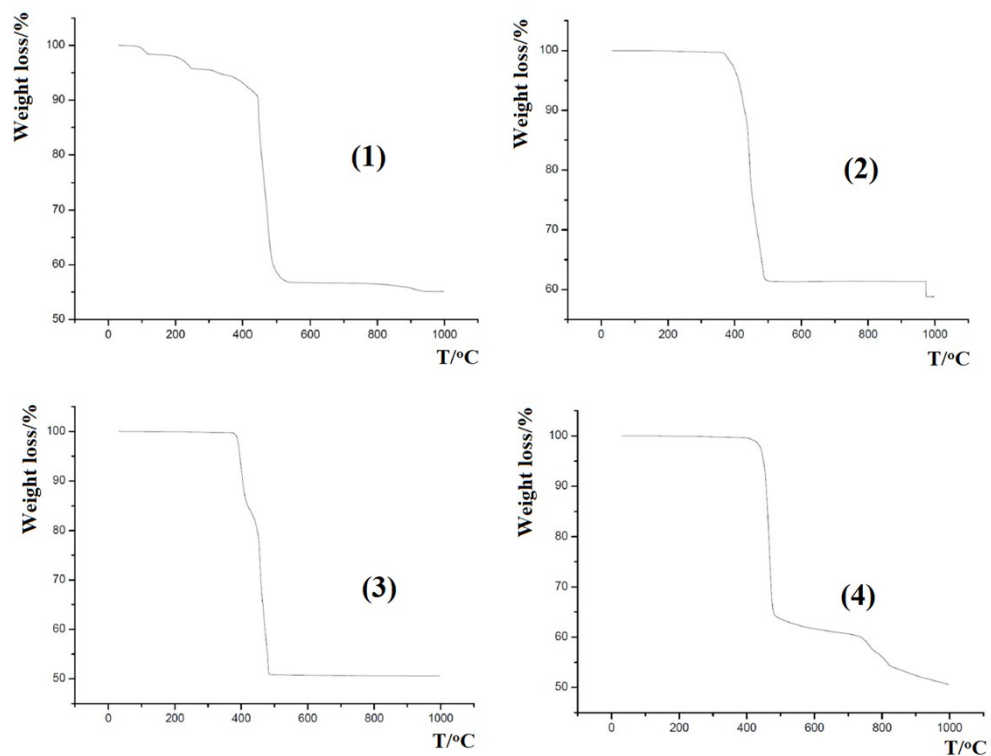
Figure S1. TGA curves for (1) - (4).
