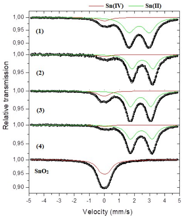
Figure S2. ^{119}\text{Sn} Mossbauer spectra of (1) - (4).
