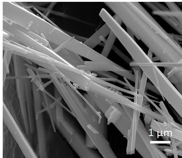
Fig. S1 SEM image of BA-4P composite
