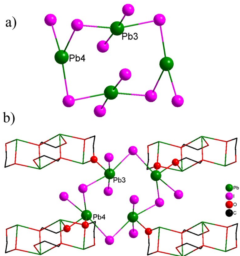
Fig. S3 (a) [\text{Pb}_4\text{I}_{10}] cluster in 2 , (b) each [\text{Pb}_4\text{I}_{10}] cluster linking with four tetra-nuclear [\text{Pb}_4\text{L}_4] complexes.
