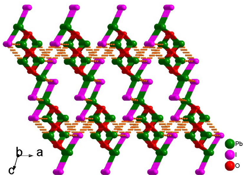
Fig. S2 3-D supramolecular network structure in 1 .
