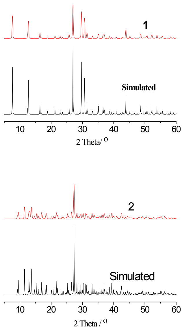
Fig. S1 Simulated and experimental powder XRD patterns of 1 and 2 .
