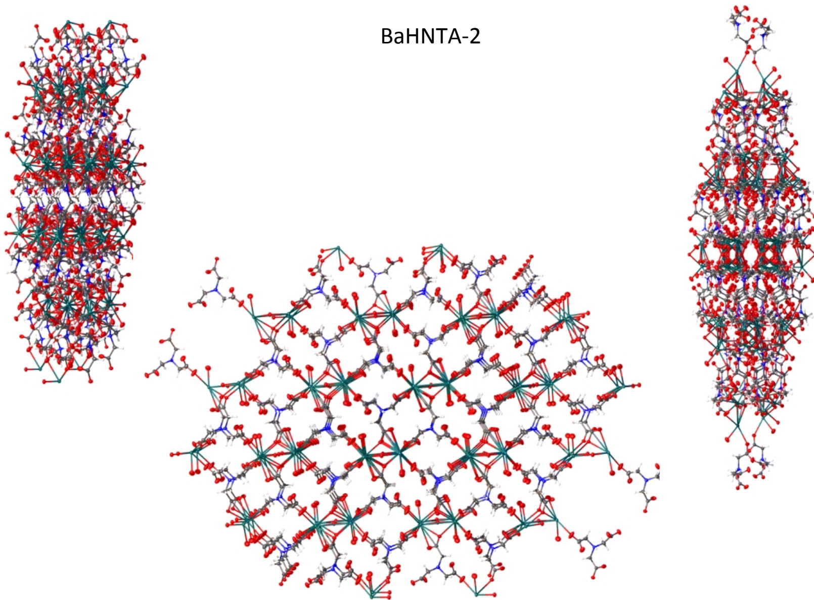
Packing along a , b , c axes (Olex2-POV-Ray representation)
