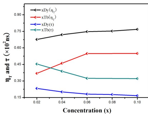
Fig. S4 Scatter plot of decay time of Ce 3+ and energy transfer efficiency from Ce 3+ to Dy 3+ and Tb 3+ .
