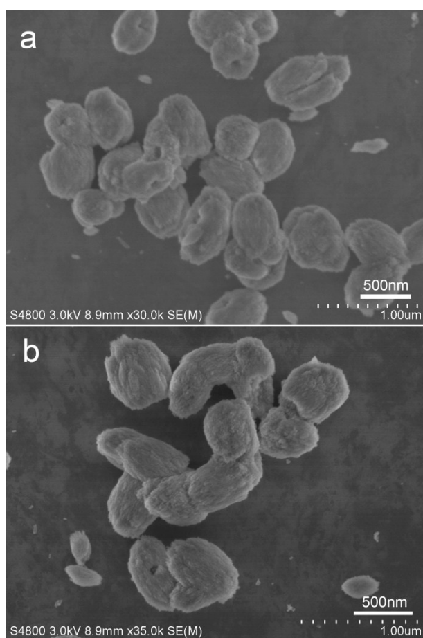
Fig. S2 SEM images of the \text{CeCO}_3\text{F}:\text{x}0.06\text{Tb}^{3+} (a), \text{CeCO}_3\text{F}:0.08\text{Eu}^{3+} (b) samples.
