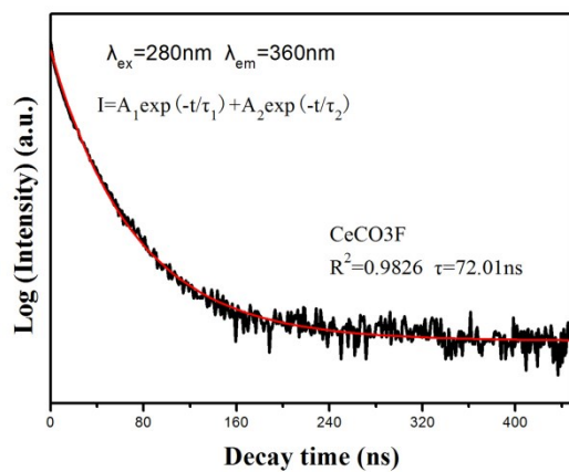
Fig. S3 Representative decay curves for the luminescence of Ce 3+ in CeCO 3 F.
