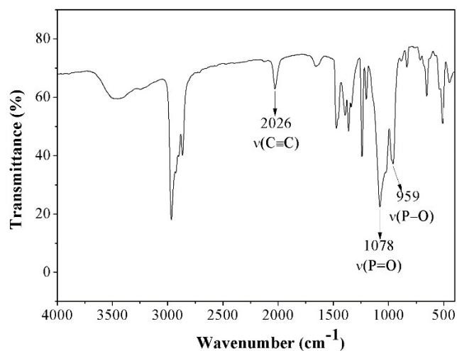
Figure S1. IR spectrum of compound 2.
