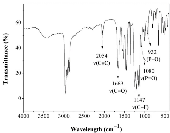
Figure S3. IR spectrum of compound 4.
