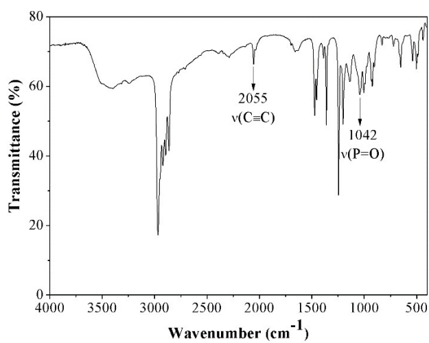
Figure S2. IR spectrum of compound 3.
