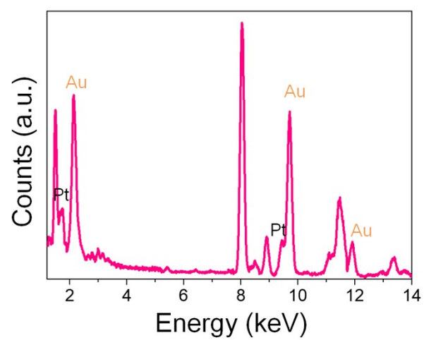
Figure S2. EDX spectrum of Au@Pt nanotriangles.
