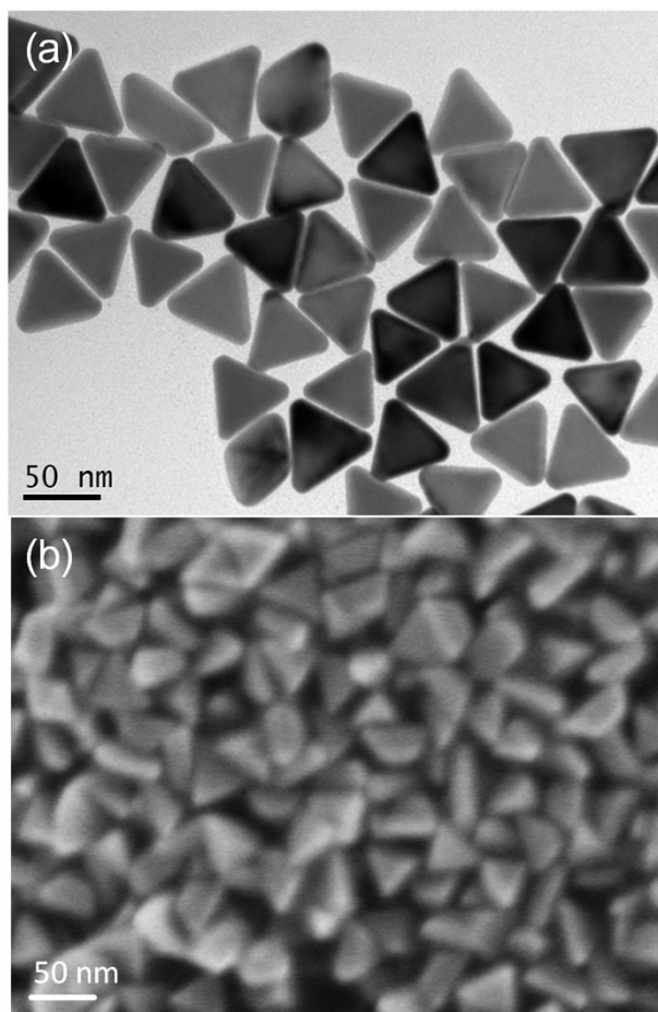
Figure S1. TEM (a) and SEM (b) images of Au nanotriangles.
