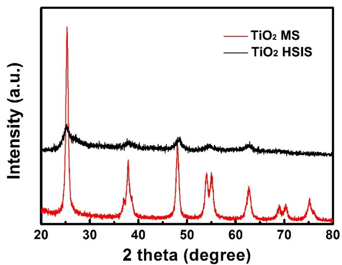
Figure S1. XRD patterns of TiO 2 HSIS and TiO 2 MS before low-temperature calcination.
