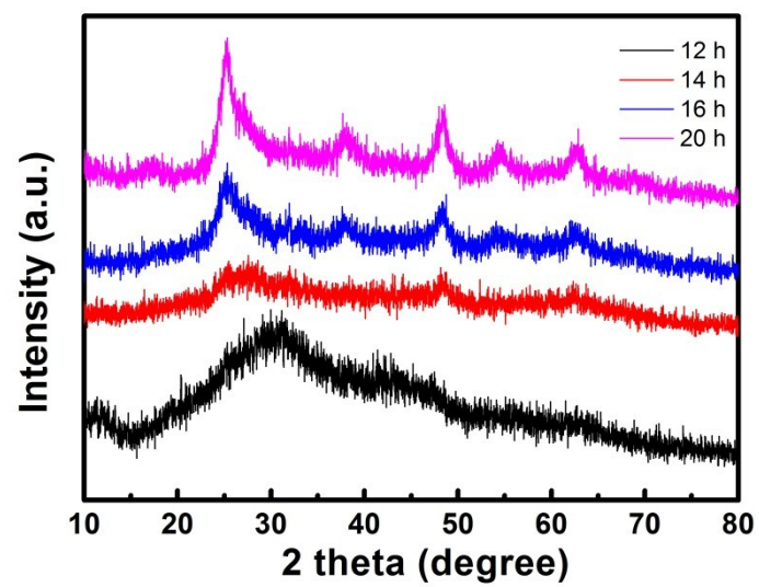
Figure S3. XRD patterns of various \text{TiO}_2 HSIS intermediates.
