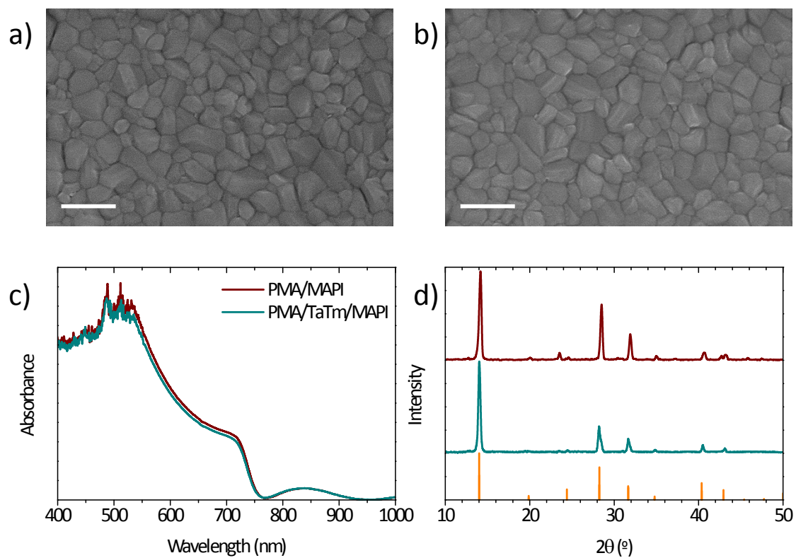
Figure S1 Scanning electron microscopy images of the surface of a MAPI film deposited on (a) PMA and (b) PMA/TaTm. (c) Optical absorption and (d) XRD patterns of the same samples (the orange lines are a reference MAPI pattern, ICSD collection code 250735).
