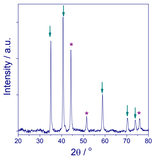
Fig. S2 XRD pattern of sample at RT after reduction at 600°C. Arrows indicate position of MnO, asterisks - Co.
