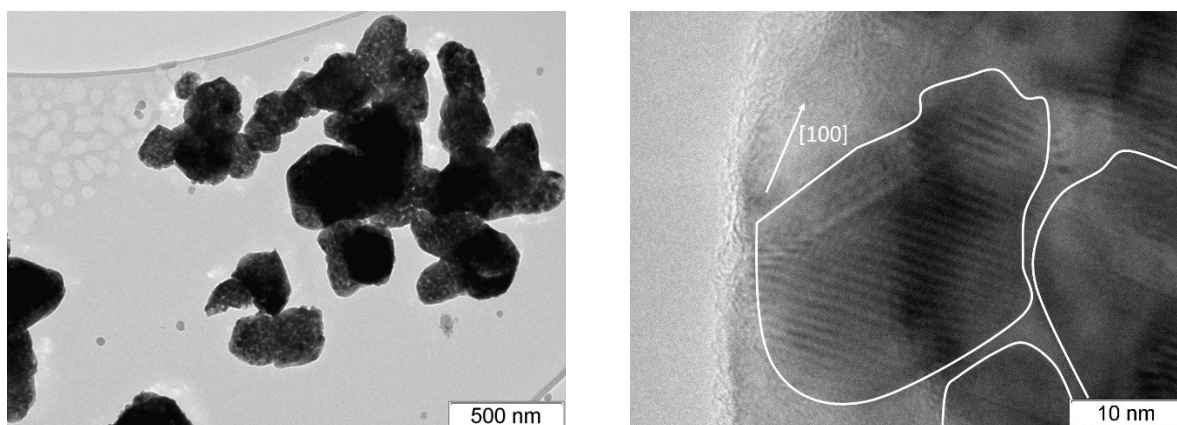
Fig. S1 TEM images for mixed Mn-Co oxides reduced at 500 °C.
