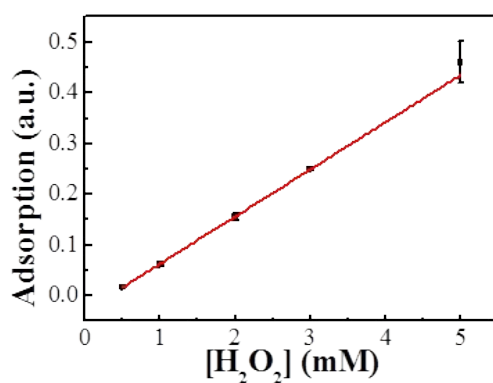
Figure S1. The calibration curve of pertitanic acid.
