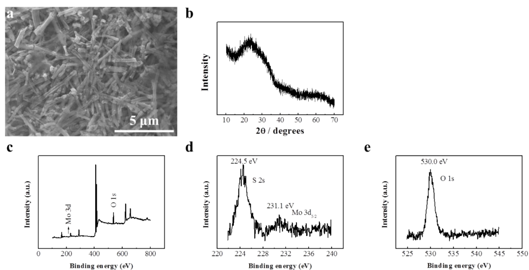
Figure S2 The SEM image (a), XRD pattern (b), XPS spectra (c-e) of \text{Fe}_2\text{O}_3 \cdot 3.9\text{MoO}_3 nanowires after reused 5 cycles: (d) S 2s and Mo 3d, and (e) O 1s.
