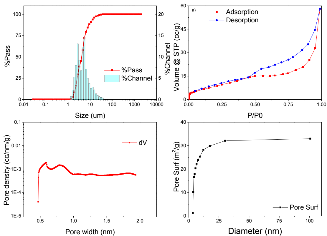
Fig. S1 The particle size distribution and multi-point BET of montmorillonite K 10 .
