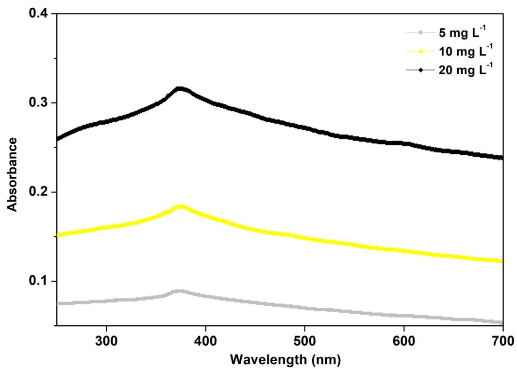
Fig. S2. UV-vis spectra of ZnO NPs in the microcosms.
