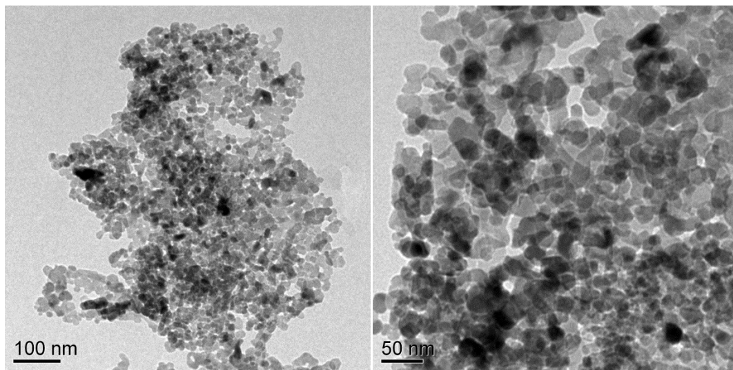
Fig. S1. Transmission electron microscopy images of stocks of ZnO NPs.
