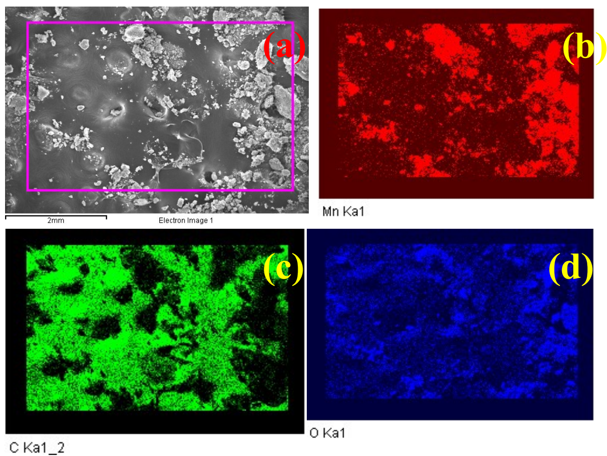
Fig. S2 Elemental mapping for \text{MnO}_2@\text{CQDs} .
