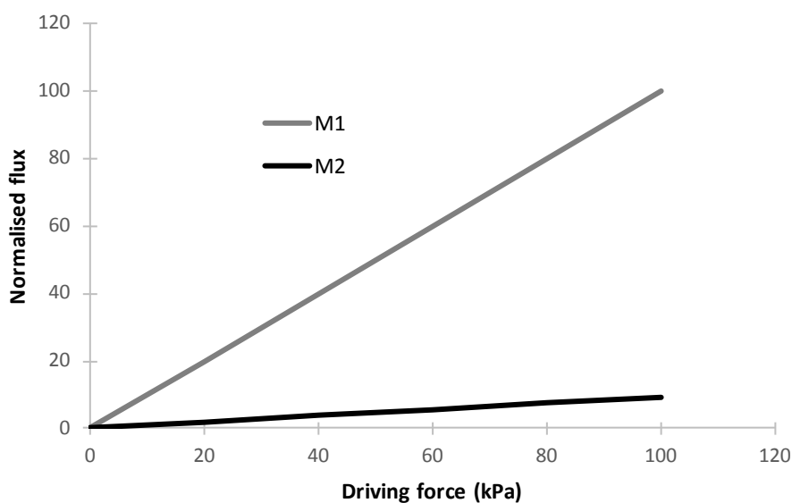
Figure 1S: Normalised flux variation with mass transfer driving force of M1 and M2 membranes
