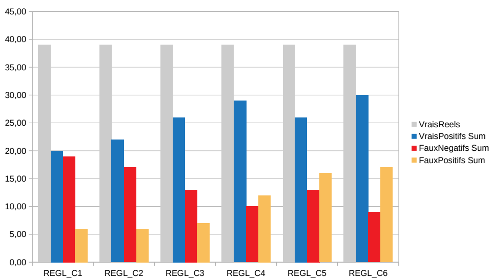
Figure S2 Selectivity / Sensitivity values for the harsh cleaning associated to Linear Regression analysis
