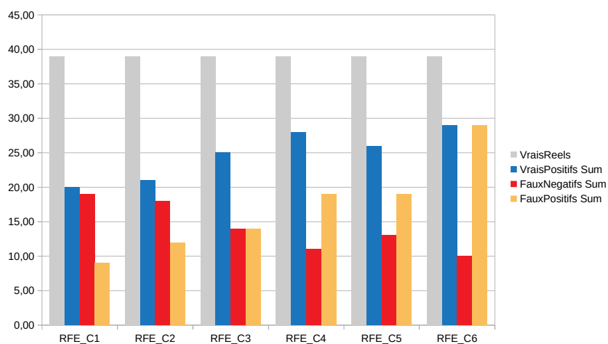
Figure S1 Selectivity / Sensitivity values for the harsh cleaning associated to RFE analysis
