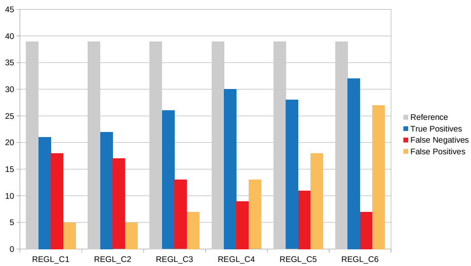
Figure S4 Selectivity / Sensitivity values for the medium cleaning associated to Linear Regression analysis
