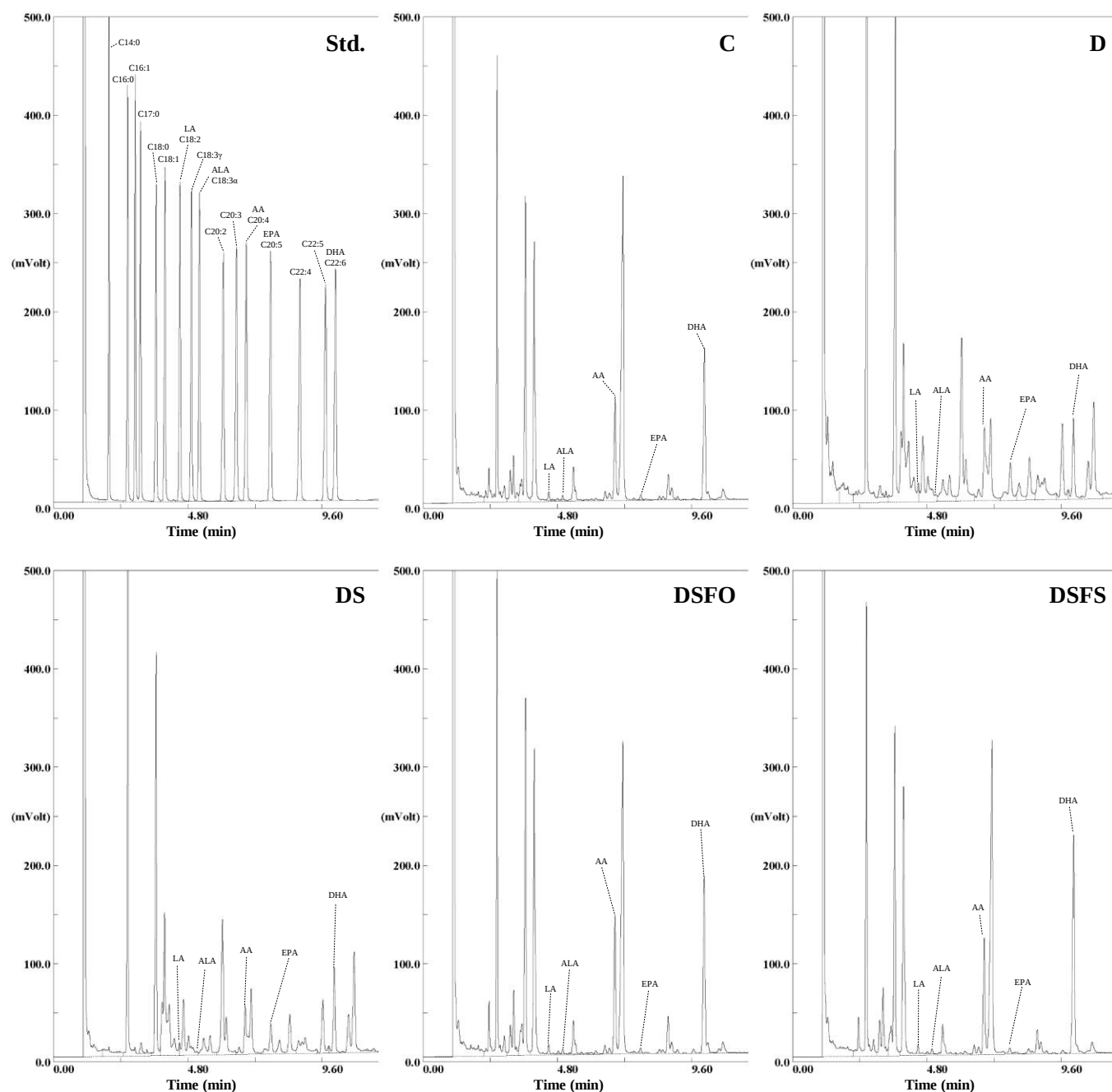
Supplemental Figure: The fatty acids GC chromatogram of prefrontal cortex.
