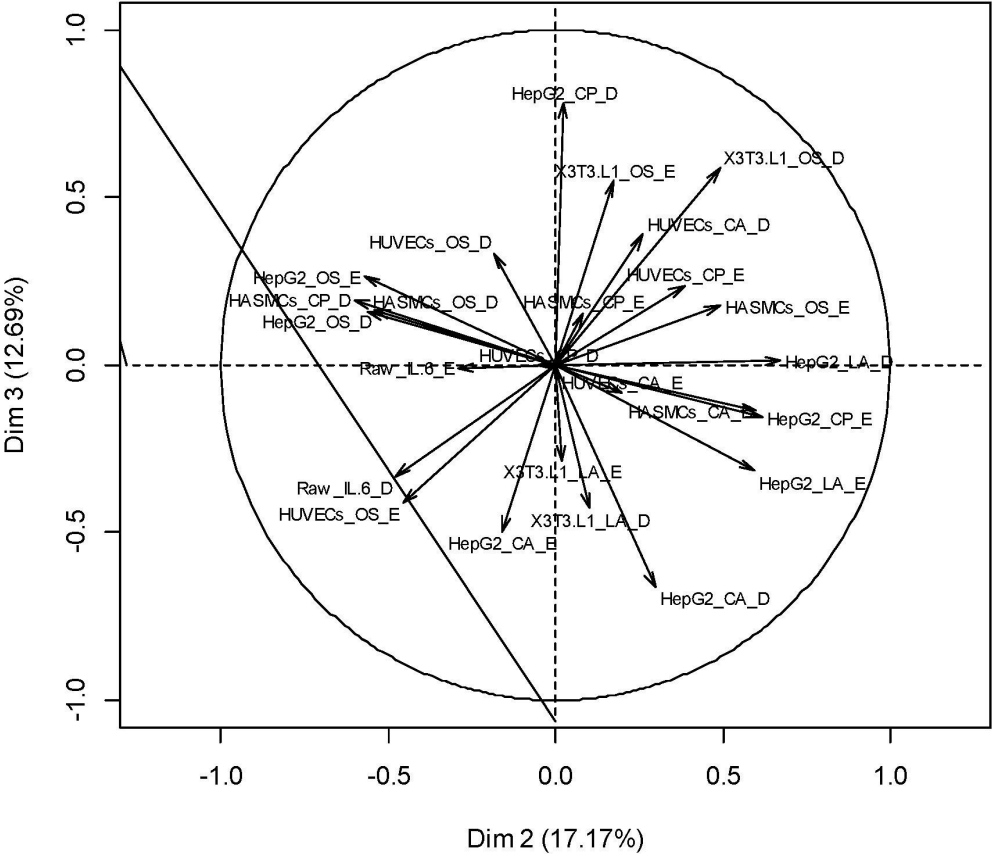
PCA_Cell tests
